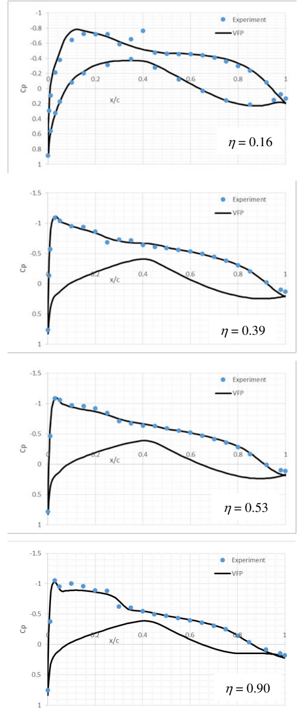
Fig 6: Comparison of measured and computed surface pressure distributions for W4. M_\infty=0.78 , \alpha = 0.0^\circ , Re_c=5.12 \times 10^6 .
