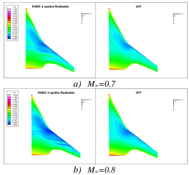
Fig 15: Comparison of the computed upper surface pressure contours for BW-11, \alpha = 0^\circ , Re_c=9 \times 10^6 .
