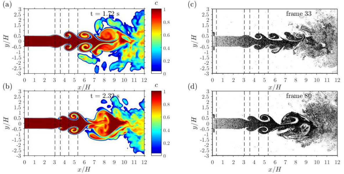
Fig. 10 - Instant concentration field: numerical (colored, a,b) and experimental PIV (black-white, c,d) results at Re=6800 .
