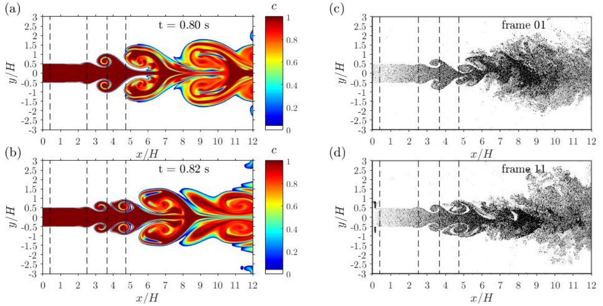
Fig. 16 - Instant concentration field: numerical (colored, a,b) and experimental PIV (black-white, c,d) results at Re=10,400 .
