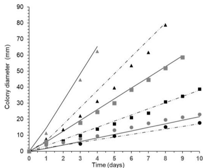
Figure 1. Fitted colony growth curves for F. asiaticum (strain 082) on wheat-based media at 35\text{ }^{\circ}\text{C} ( \blacktriangle , 0.98\text{ }a_w ; \blacksquare , 0.95\text{ }a_w ; \bullet , 0.93\text{ }a_w ) and 25\text{ }^{\circ}\text{C} ( \triangle , 0.98\text{ }a_w ; \square , 0.95\text{ }a_w ; \circ , 0.93\text{ }a_w ) fitted to Baranyi model (—, 30\text{ }^{\circ}\text{C} ; ----, 15\text{ }^{\circ}\text{C} ).
