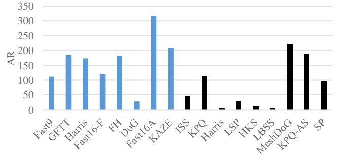
(a) (b) Fig. 9 Evaluating 2D (blue) and 3D (black) keypoint detectors on the SpaceTime dataset. (a) RR (b) AR.
