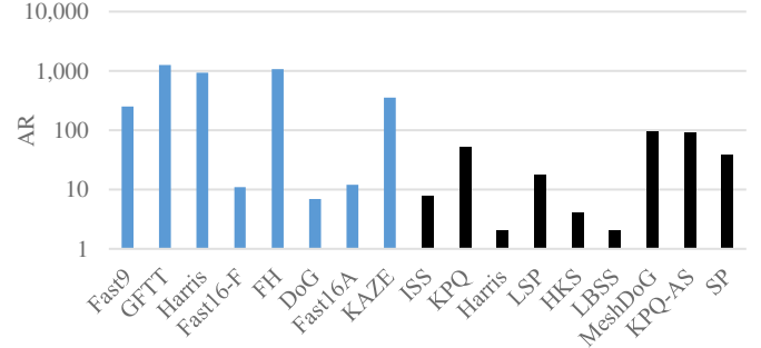
(a) (b) Fig. 8 Evaluating 2D (blue) and 3D (black) keypoint detectors on the Kinect dataset. (a) RR. (b) AR.
