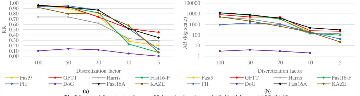
Fig. 2 Impact of discretization factor on 2D keypoint detection on the Oakland dataset. (a) RR. (b) AR.
