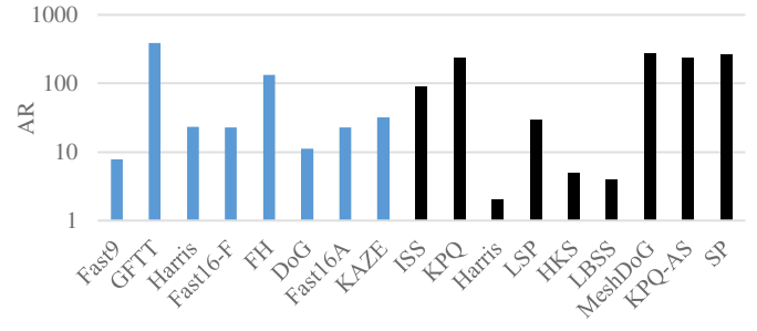
(a) (b) Fig. 7 Evaluating 2D (blue) and 3D (black) keypoint detectors on the Laser Scanner dataset. (a) RR. (b) AR.
