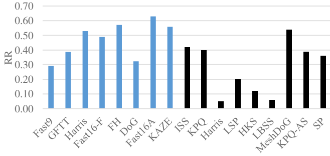
(a) (b) Fig. 9 Evaluating 2D (blue) and 3D (black) keypoint detectors on the SpaceTime dataset. (a) RR (b) AR.
