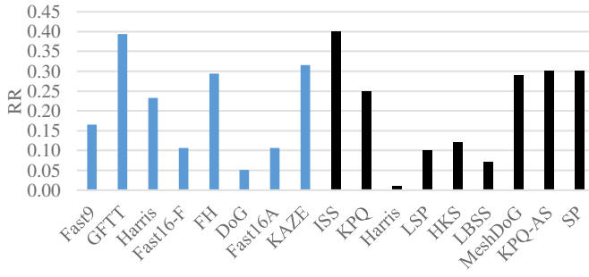
(a) (b) Fig. 7 Evaluating 2D (blue) and 3D (black) keypoint detectors on the Laser Scanner dataset. (a) RR. (b) AR.
