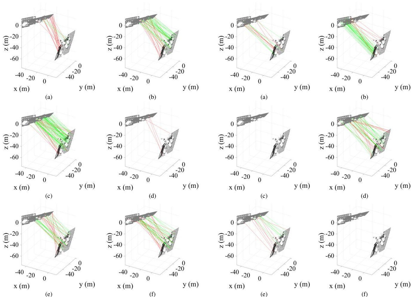
Fig. 18 Example presenting the overall top AUC performing cross / single dimensional feature correspondences on two scenes of the Oakland dataset under 1/8 subsampling rate difference (a) ISS/ FREAK (b) ISS/ SURF (c) uniform/ SURF (d) GFTT/ BRISK (e) ISS/ KAZE (f) FH/ SIFT (green and red lines present the TP and FP correspondences, figure is best seen in colour).
