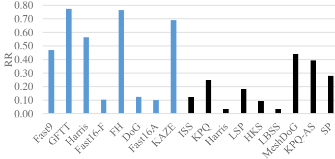
(a) (b) Fig. 8 Evaluating 2D (blue) and 3D (black) keypoint detectors on the Kinect dataset. (a) RR. (b) AR.
