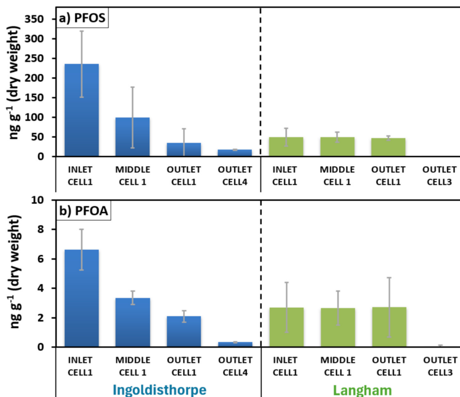
Fig. 3. Dry weight concentrations of PFOS (a) and PFOA (b) in sediment samples at different sampling points in Ingoldisthorpe (blue) and Langham (green) surface flow treatment wetlands.
