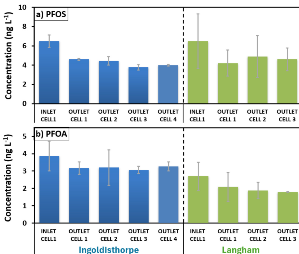
Fig. 2. Mean concentration of PFOS (a) and PFOA (b) in water samples at different sampling points of Ingoldisthorpe (blue) and Langham (green) surface flow treatment wetlands.
