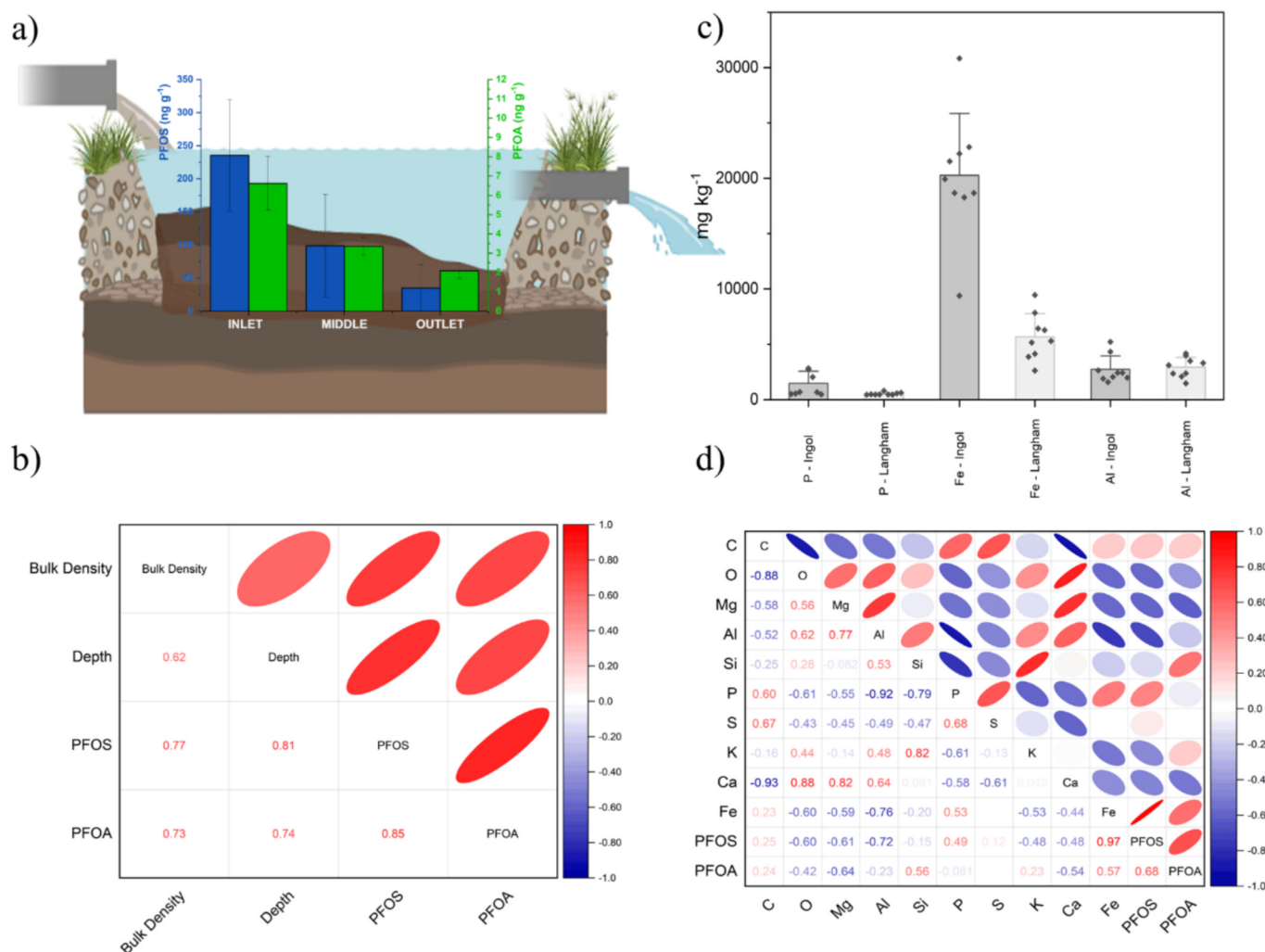
Fig. 4. Variation in sediment depth and mean concentrations of PFOS (blue) and PFOA (green) in \text{ng g}^{-1} (dry weight) in sediment samples collected at different points within cell 1 of the Ingoldisthorpe wetland (a). Pearson correlations between PFOS and PFOA concentrations, bulk density, and sediment depths (b). Statistical representation of dry weight concentration of total phosphorus (P), total iron (Fe), and total aluminium (Al) in sediment samples from the first cell of the Ingoldisthorpe (dark grey) and Langham (light grey) wetland (c). Pearson correlations between PFOS and PFOA concentrations in sediments and sediment chemical composition (d).
