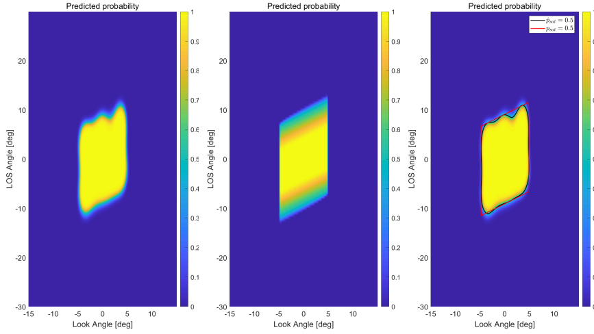
Fig. 10 The predicted probability distribution (Left), the true probability distribution (Center), and the decision boundary (Right) after 60th iteration
