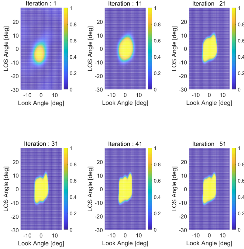
Fig. 8 Evolution of the predicted probability distribution \hat{p}_{sat}(\theta)
