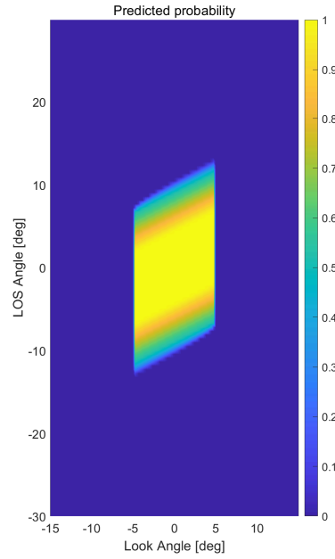
Fig. 7 True satisfaction probability function p_{sat}(\theta) for the capture region against stochastic target
