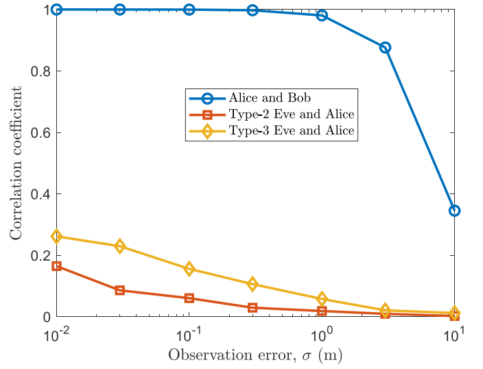
Fig. 4. Performance of CLS against two types Eves, where x-coordinate is the different levels of observing noises and y-coordinate is the correlation coefficients.
