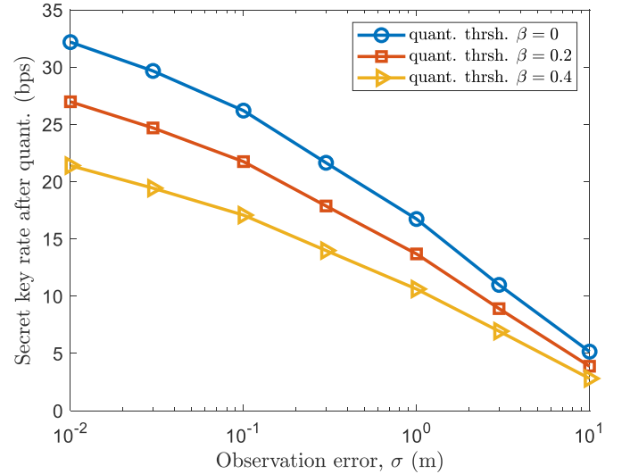
Fig. 7. Secret key rate after key quantization of our proposed CLS.
