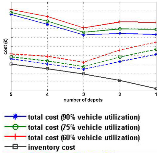
Figure 4a. Logistics costs related to number of depots and vehicle utilization parameters for centre o - gravity locations
