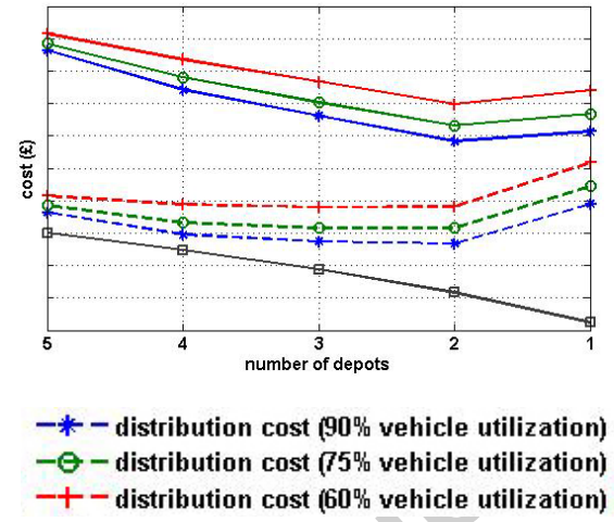
Figure 4b. Logistics costs related to number of depots and vehicle utilization parameters for original locations.
