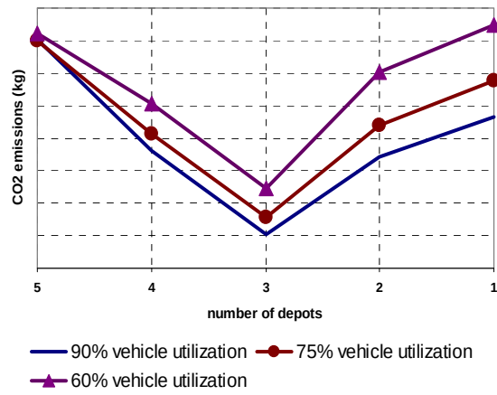
Figure 6a. Total CO 2 emissions from transport and electricity related to number of depots and vehicle utilization parameters for centre of gravity scenario.
