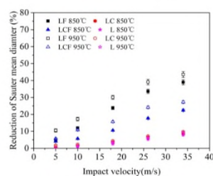
Mean diameter after impact breakage versus impact velocity
