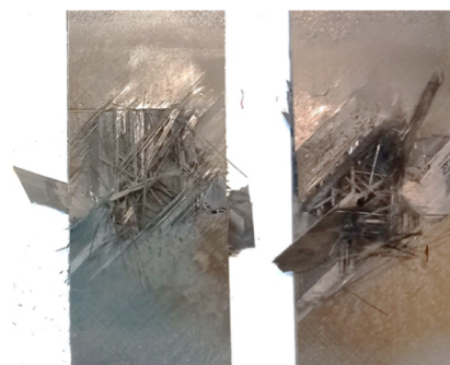
b) Post-TAL testing
