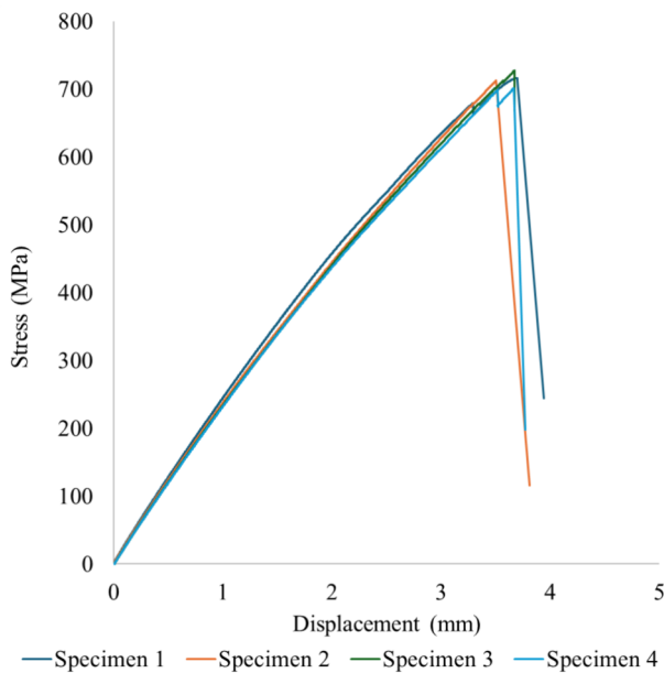
Fig. 3. Stress-displacement curves from four TAL tests.
