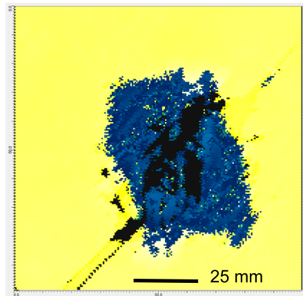
a) Ultrasound scan of a typical TAL specimen
