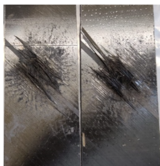
a) Post-strike, pre-TAL testing
