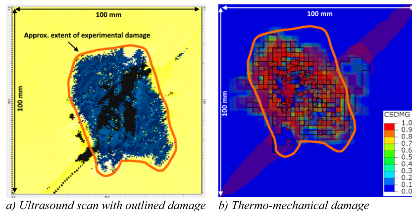
Fig. 5. Comparison of experimental ultrasound scan and thermo-mechanical damage predictions where colours represent delamination damage.
