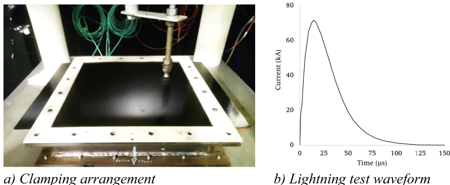
Fig. 1. Laboratory lightning strike test with a) clamping used and b) waveform used.
