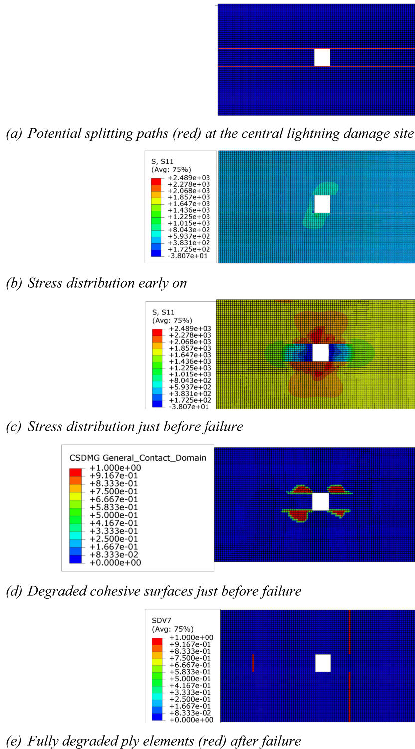
Fig. 6. FE results in the 3 rd 0° ply of the TAL model.
