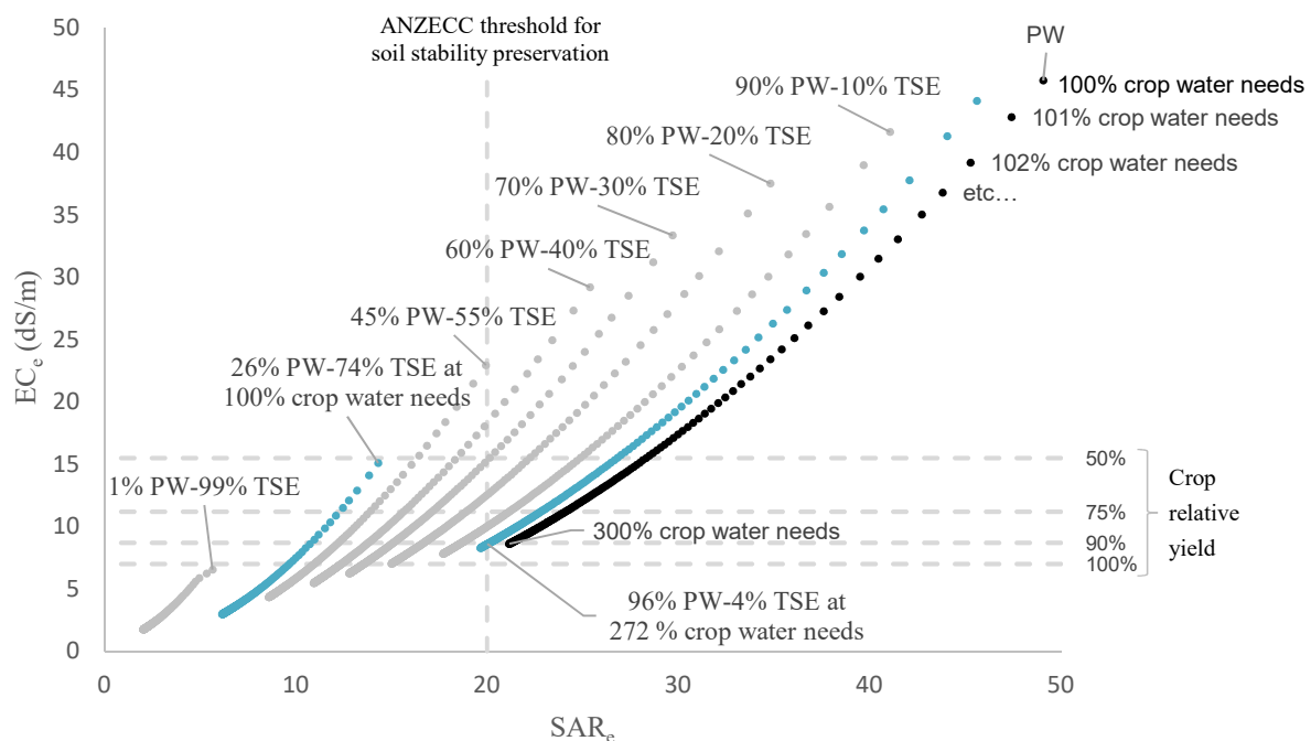
Figure 2. Long-term EC_e and SAR_e following irrigation of sugar beet with different blends of PW diluted with TSE (from 100% PW down to 1% PW + 99% TSE) and with different irrigation amounts (from 100% up to 300% of the crop water needs).
