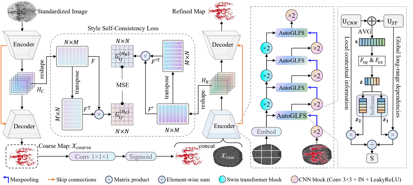
Fig. 3. Schematic of CESAR highlighting its key components: the coarse-to-fine backbone (C2F), style self-consistency loss (SSL), and automatic global and local feature selection module (AutoGLFS). The C2F framework allows fine-grained segmentation, while the SSL boosts adaptability to multi-centric data. The AutoGLFS selectively fuses the long-range dependencies and local contexts.
