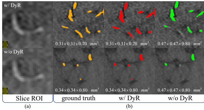
Fig. 8. Cerebrovascular segmentation results of TOF-MRA images with and without DyR, showing (a) ROI resampled with and without DyR, and (b) cerebrovascular segmentation results by CESAR in resampled images with and without DyR.
