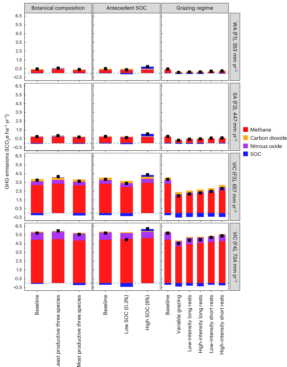
Fig. 3 | Average annual net GHG emissions (points) and gross GHG emissions (bars) derived from SOC, carbon dioxide ( \text{CO}_2 ), enteric methane ( \text{CH}_4 ) and nitrous oxide ( \text{N}_2\text{O} ) for several botanical compositions (first column), antecedent SOC levels (second column) and grazing regimes (third column). Row titles depict farm abbreviation (F1–4) and long-term average annual rainfall ( \text{mm yr}^{-1} ) across regions, with Western Australia (WA), South Australia (SA) and Victoria (VIC). Least and most productive three species represent swards
