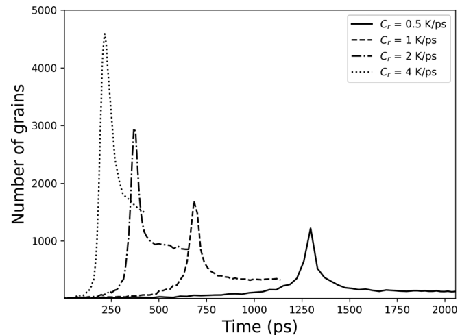
FIG. 10. Number of grains vs time.
