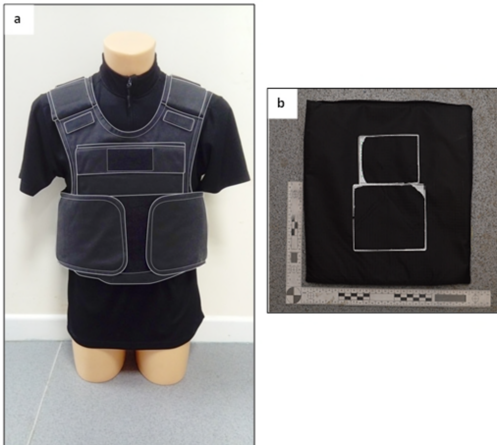
Figure 1: a) Typical police polo shirt with carrier vest over the top and b) standard UK ballistic test panel of HG1/A + KR1 body armour
