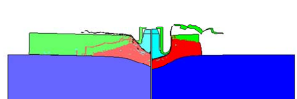
Figure 8: Computational results showing the initial stages of penetration into the ceramic-faced polycarbonate. The left hand side of the images shows the results from the 85 mm tile whereas the right hand side of the images shows the results from 33mm tile. The depth of the polycarbonate has been truncated for clarity.
