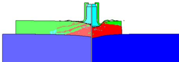
Figure 8: Computational results showing the initial stages of penetration into the ceramic-faced polycarbonate. The left hand side of the images shows the results from the 85 mm tile whereas the right hand side of the images shows the results from 33mm tile. The depth of the polycarbonate has been truncated for clarity.
