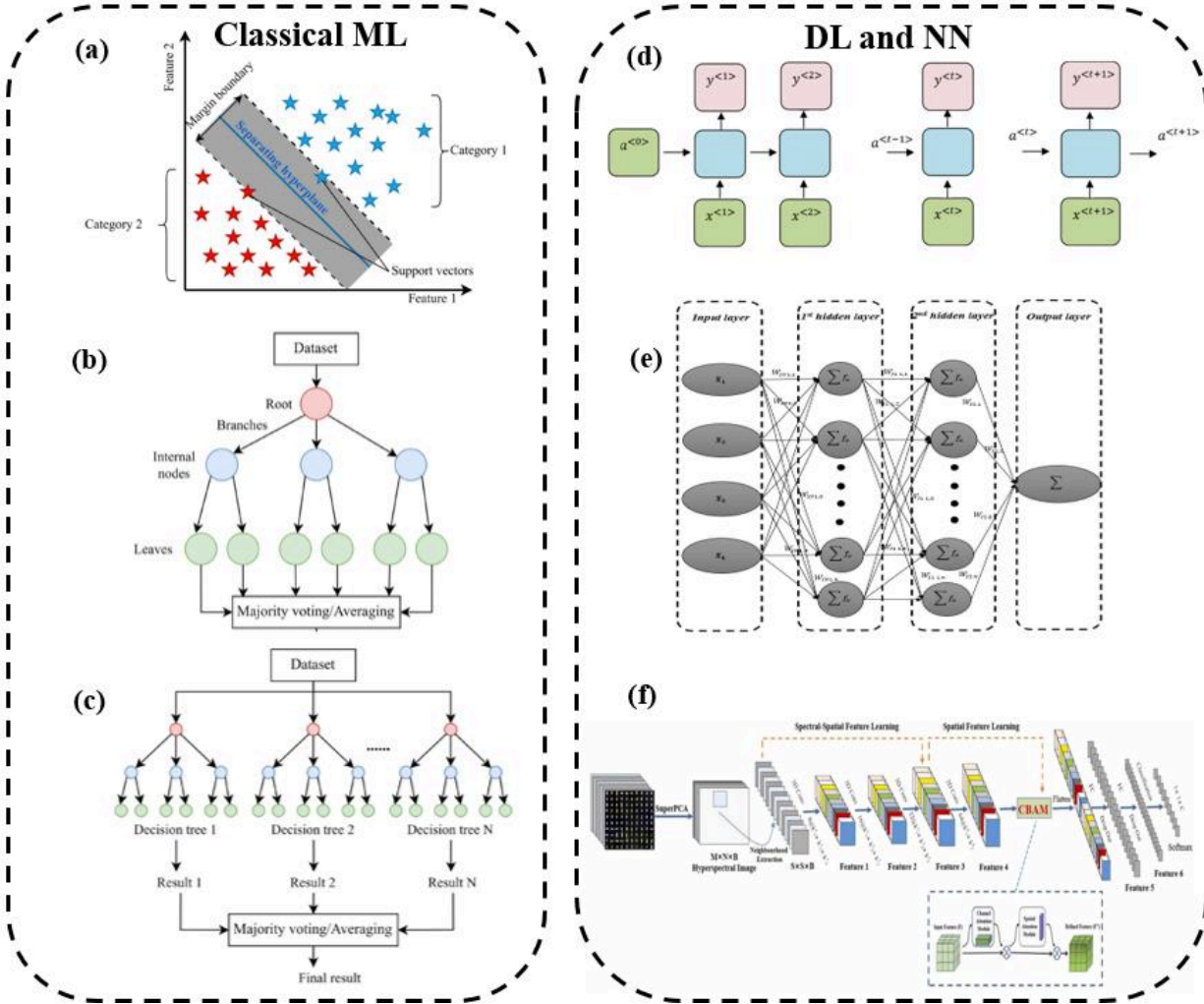
Figure2. Comparison of Classical Machine Learning and Deep Learning Architectures: (a) Support Vector Machine (SVM) classifier illustrating decision boundary and support vectors; (b) Decision Tree model with hierarchical data splits; (c) Random Forest ensemble model combining multiple decision trees for robust prediction (Reproduced from Lin et al., 2023); (d) Recurrent Neural Network (RNN) for sequential data processing (Reproduced from Dhiman et al., 2021); (e) Feedforward Neural Network with multiple hidden layers; (f) Convolutional Neural Network (CNN) (Reproduced from Wang et al., 2024).
