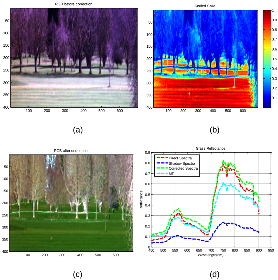
Figure 12 (a) the RGB image before correction ( I_{NP} ), (b) scaled_SAM result, (c) the RGB after correction and (d) the plot of shadow spectra before and after correction with respect to direct spectra.
