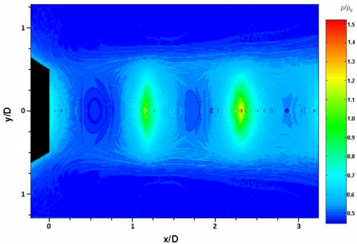
(a) Background-oriented schlieren
