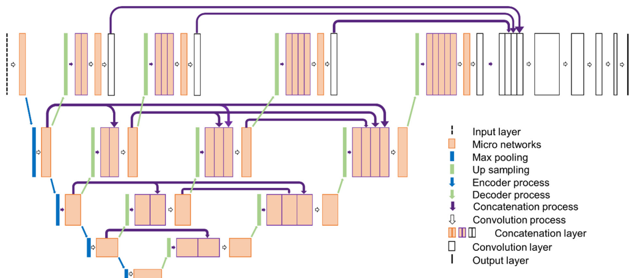
Figure 4. The proposed rock segmentation network (NI-U-Net++).
