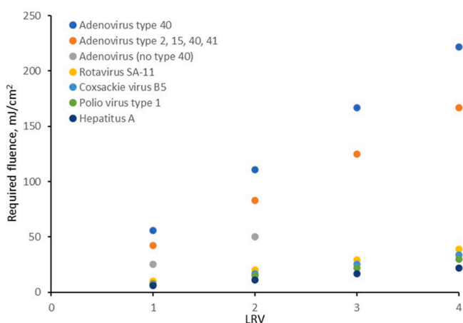
Fig. 2. Required fluence (or dose in \text{mJ}/\text{cm}^2 ) for virus inactivation by UV (Hijnen et al., 2006).
