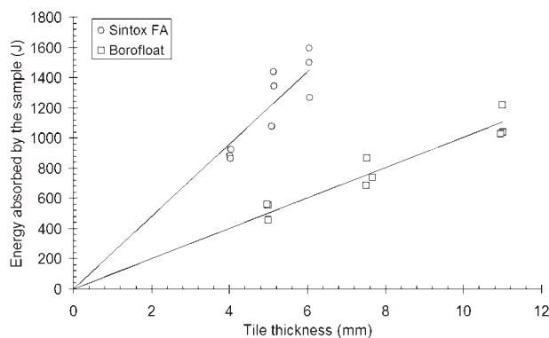
7 Energy dissipated by tiles with increasing thickness
