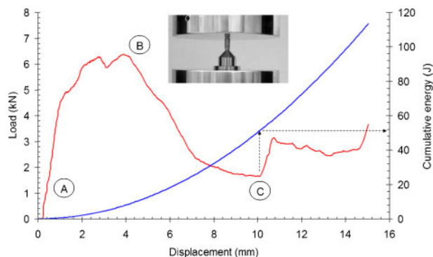
5 Compression of bullet into conically shaped die: load–displacement and cumulative energy–displacement
