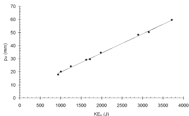
6 Depth of penetration into aluminium alloy (6082-T651) plate with varying bullet kinetic energy
