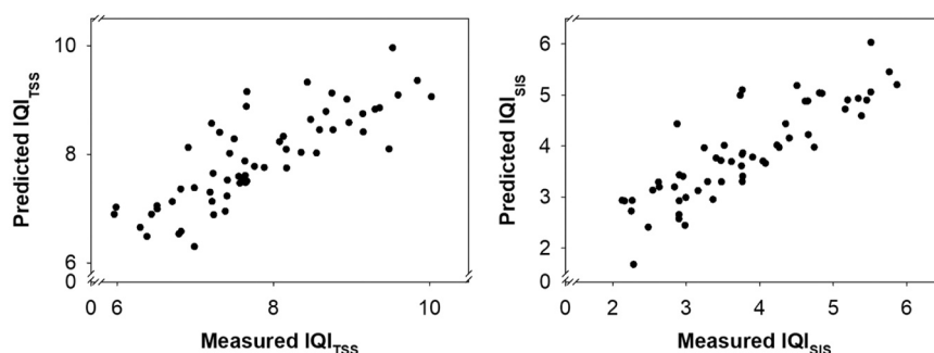
Fig. 4. Predicted vs. measured values for internal quality index (IQI) attributes using visNIRS. Models were created using 'Kent' mangoes from Peru and the Dominican Republic.
