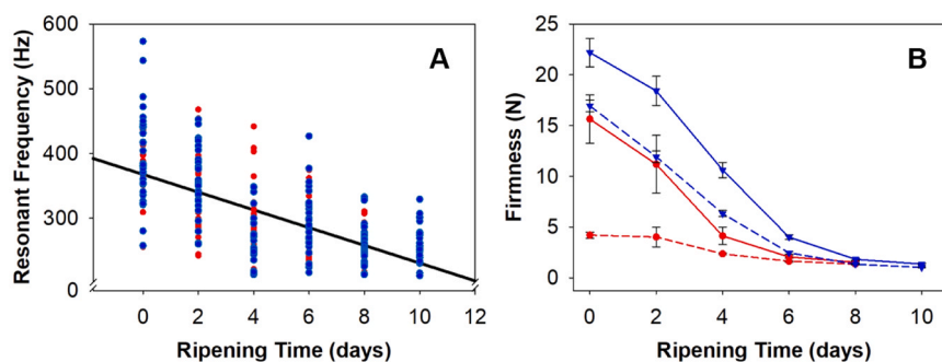
Fig. 3. Relationships between the resonant frequency (A) and destructively measured firmness (B). A: Linear correlation between resonant frequency, measured by LDV, and ripening time in 'Kent' (blue) and 'Keitt' (red) mangoes. Pearson's correlation coefficient indicated a negative linear correlation, with r = -0.65 and p < 0.001 . B: Approximately exponential decreases are seen through time for both the inner (dashed) and outer (solid) pulp firmness in 'Kent' (blue) and 'Keitt' (red) mangoes.
