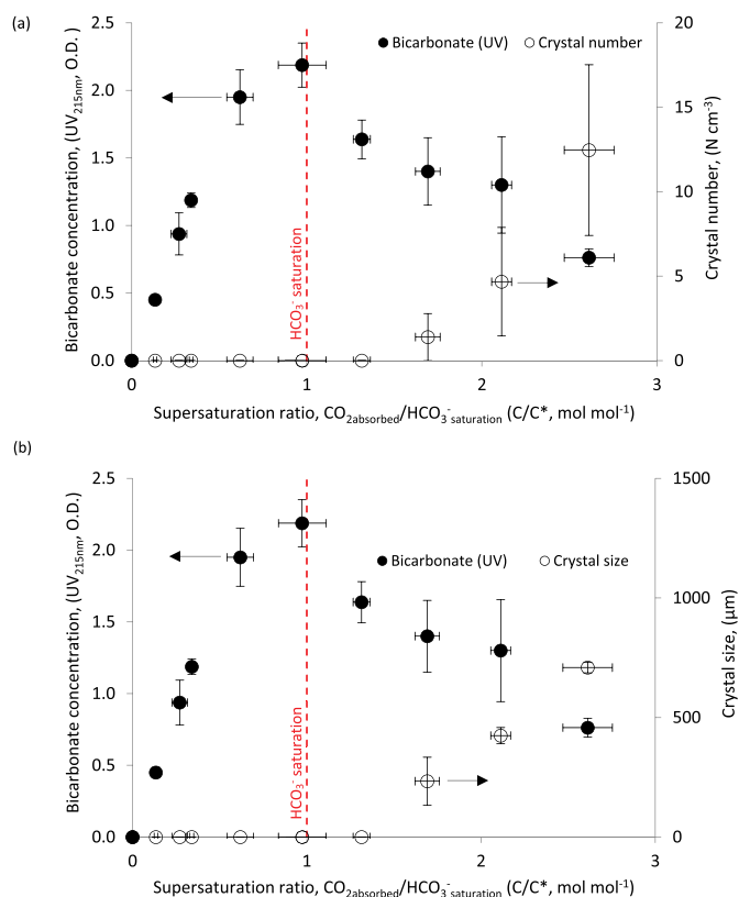
Fig. 7. Transition in (a) crystal number; and (b) crystal size, determined at progressive levels of supersaturation (saturation demands conversion of 1.5 M \text{CO}_2 into \text{HCO}_3^- ) for an \text{NH}_3 concentration of 3.3 M. Bicarbonate concentration shown for reference as this is important for induction. Error bars indicate standard deviation obtained from sacrificial experiments carried out in triplicate for each ammonia concentration.
