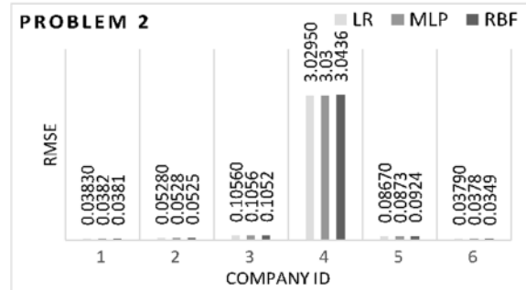
Figure 5: RMSE obtained with the three models for Problem 2.
