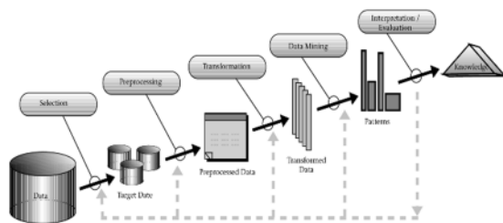
Figure 1: Data Mining as a step in the process of Knowledge Discovery (Fayyad, Piatetsky-Shapiro & Smyth 1996).
