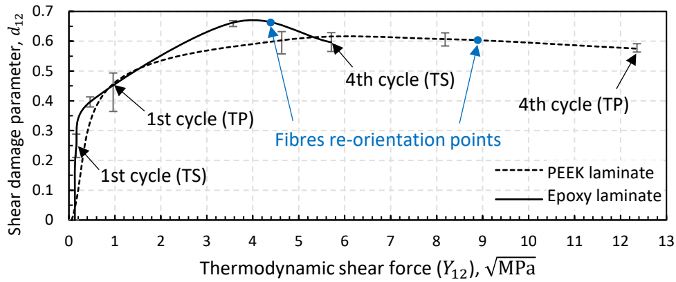
Figure 6. Shear damage parameter ( d_{12} ) evolution during \pm 45^\circ tensile cyclic testing of 977-6/T800 (solid line) and TC1200/IM7 (dashed line); The re-orientation points have been transferred from the blue points identified in Figure 4(a).
