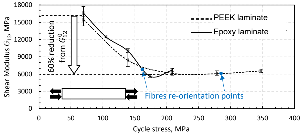
Figure 5. Shear modulus evolution versus applied stress ( 2\sigma_{12} ; values in Table 1) for (\pm 45^\circ) tensile cyclic testing 977-6/T800 (solid line) and TC1200/IM7 (dashed line); The re-orientation points have been transferred from the blue points identified in Figure 4(a).
