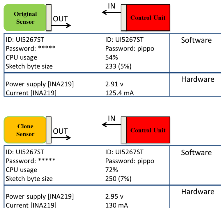
Figure 19. Reading byte between two modules.
