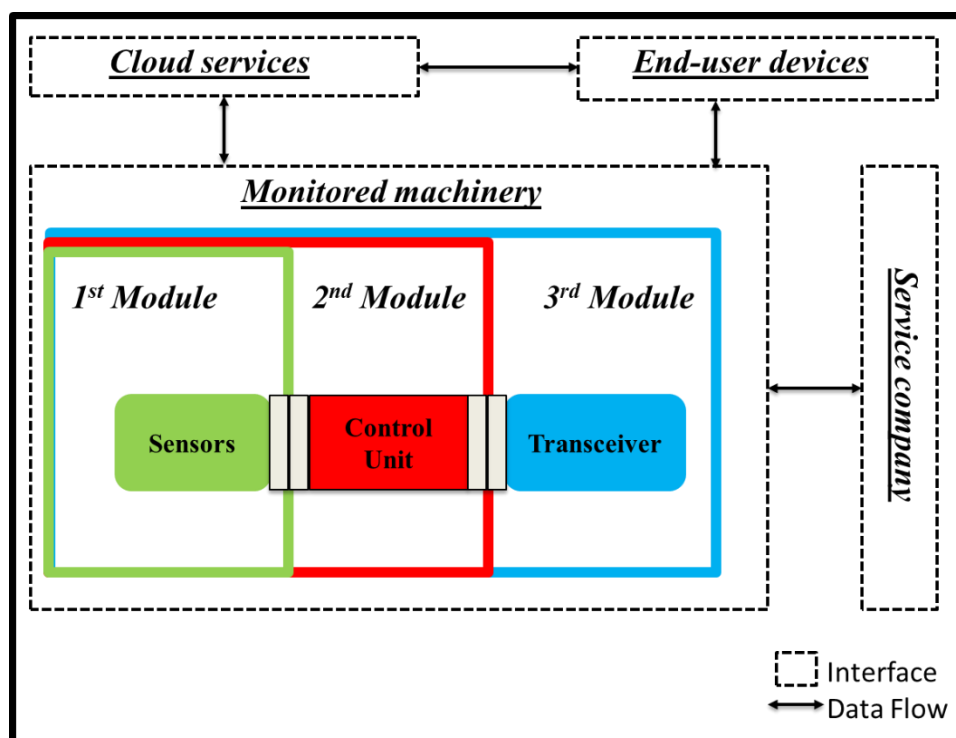
Figure 10. The IoT DAQ for legacy production machinery.
