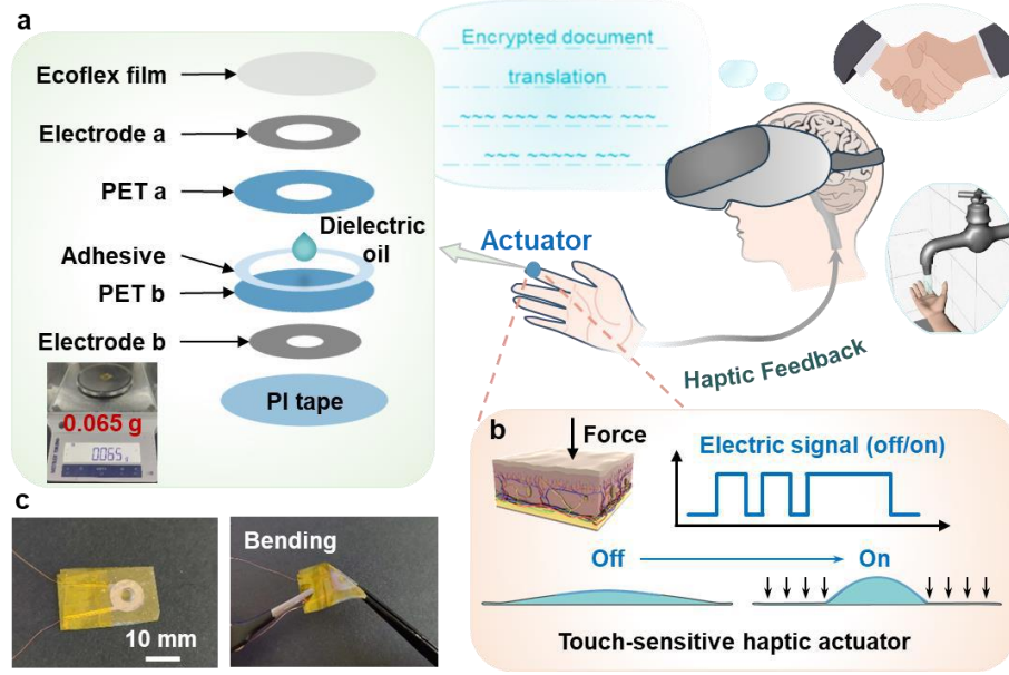
Fig. 1 Application and structure of the haptic actuator. (a) The composition of the haptic actuator. (b) Signal transmission via the on/off state of the voltage-driven actuator. (c) Photograph of the actual haptic actuator.
