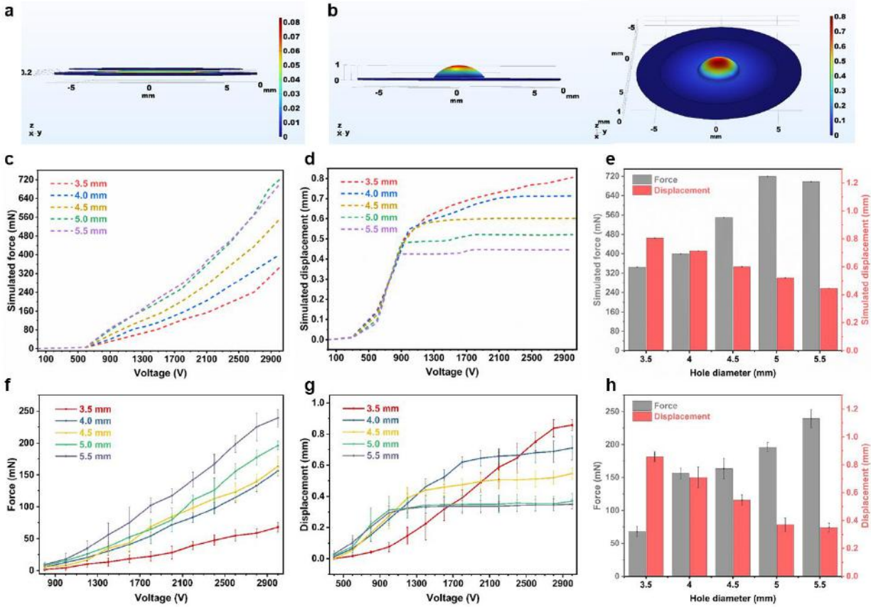
Fig. 4. Measured and simulated force and displacement of haptic actuators with different aperture designs. (a) and (b) Model simulations of the haptic actuator's force and displacement. (c) and (d) Simulated force and displacement of the haptic actuator as a curve of voltage. (e) Summary of the simulated force and displacement of the haptic actuator at 3000 V. (f) and (g) Measured force and displacement of the haptic actuator as a curve of voltage. (h) Summary of the measured force and displacement of the haptic actuator at 3000 V.
