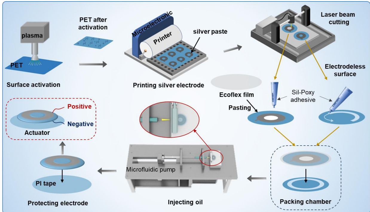
Fig. 2 Schematic of the fabrication process for the haptic actuator.
