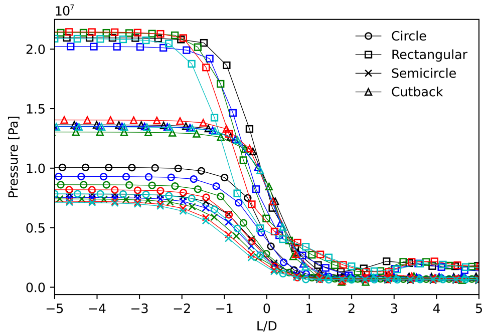
Figure 6. Pressure drop alongside the L/D distance from the orifice. Color: black ( L/D = 0.5 ), blue ( L/D = 0.69 ), green ( L/D = 0.89 ), red ( L/D = 1.08 ), and cyan ( L/D = 1.28 ).
