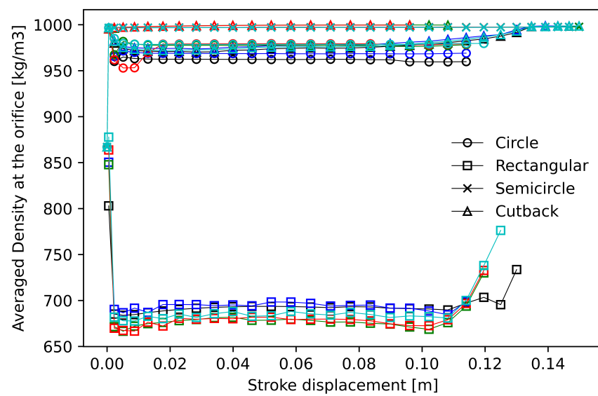
Figure 8. Density at the orifice probe alongside stroke displacement for various orifice shapes and lengths. Color: black L/D = 0.5 , blue L/D = 0.69 , green L/D = 0.89 , red L/D = 1.08 , and cyan L/D = 1.28 .
