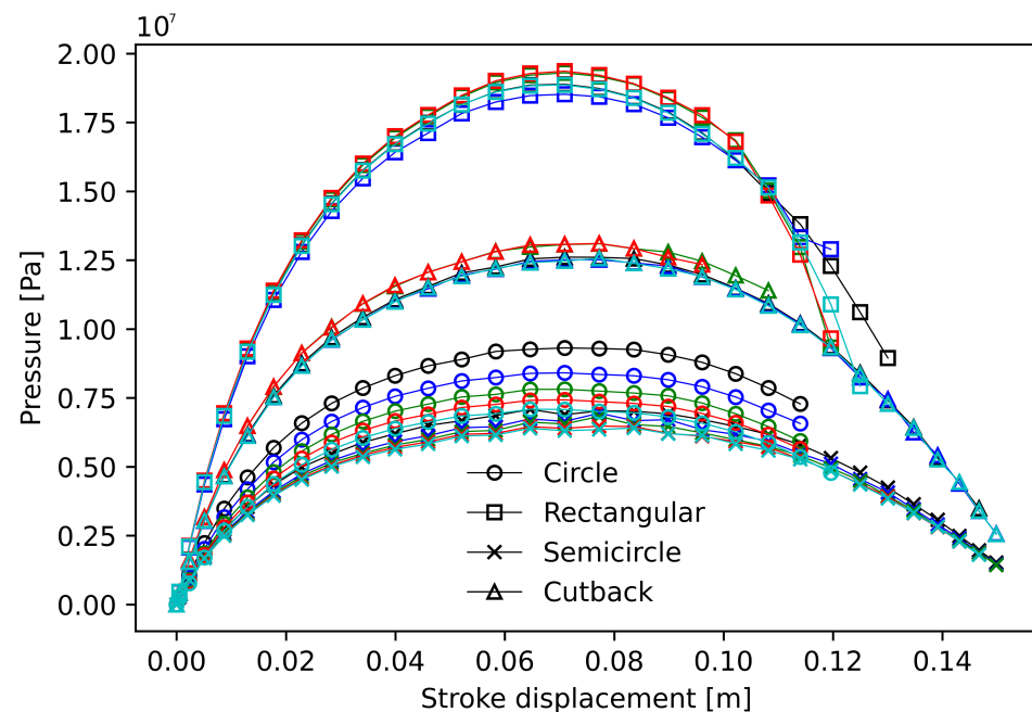
Figure 5. Pressure drop alongside stroke displacement for various orifice shapes and lengths. Color: black ( L/D = 0.5 ), blue ( L/D = 0.69 ), green ( L/D = 0.89 ), red ( L/D = 1.08 ), and cyan ( L/D = 1.28 ).
