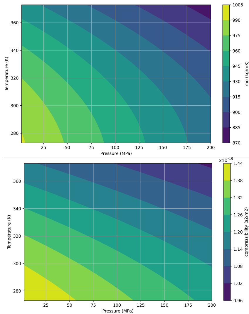
Figure 2. Equation of state for the oil: the density ( top ) and compressibility ( bottom ), \psi , as function of pressure and temperature.
