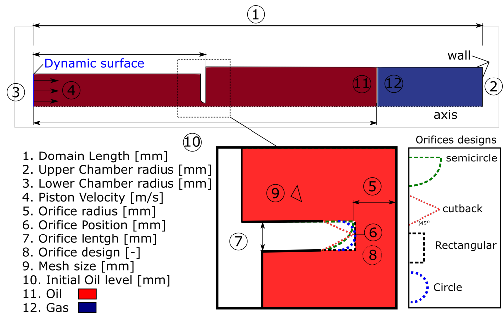
Figure 1. Geometry schematic of shock absorber.
