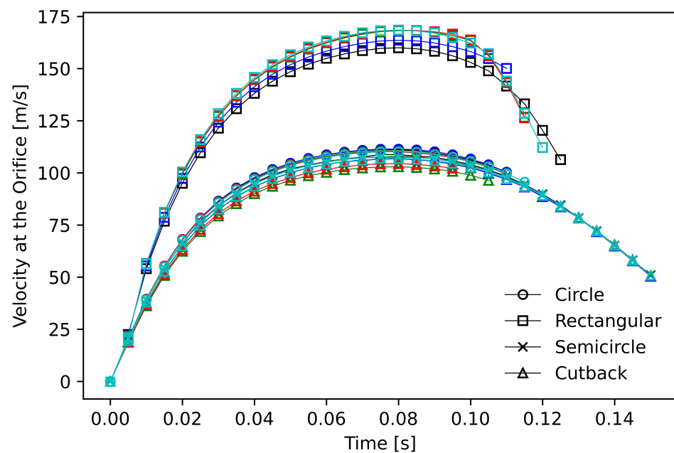
Figure 7. Orifice velocity alongside stroke displacement for various orifice shapes and lengths. Color: black L/D = 0.5 , blue L/D = 0.69 , green L/D = 0.89 , red L/D = 1.08 , and cyan L/D = 1.28 .
