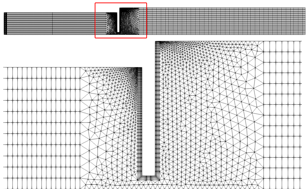
Figure 4. Computational grid overview ( top ) and in detail ( bottom ).
