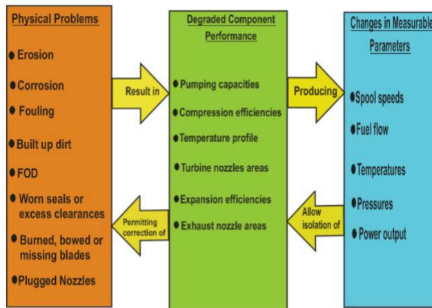
Figure 7 Engine fault and parameter relationship
