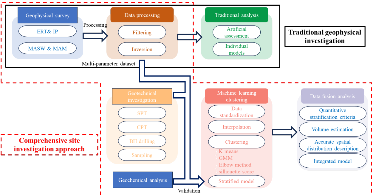
Fig. 1. Comparison of the traditional geophysical investigation approach and the comprehensive site investigation approach used in this study.
