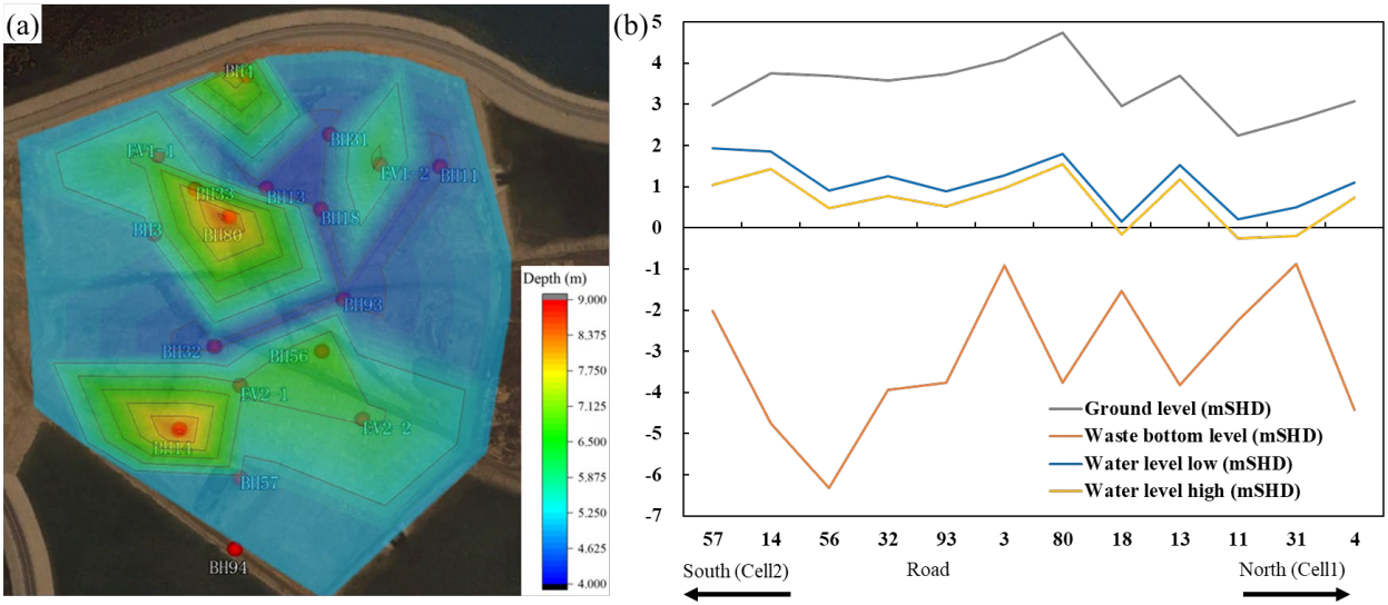
Fig. 4. Underground information obtained from boreholes and water standpipes: (a) waste depth; (b) thickness of waste and groundwater level (mSHD).
