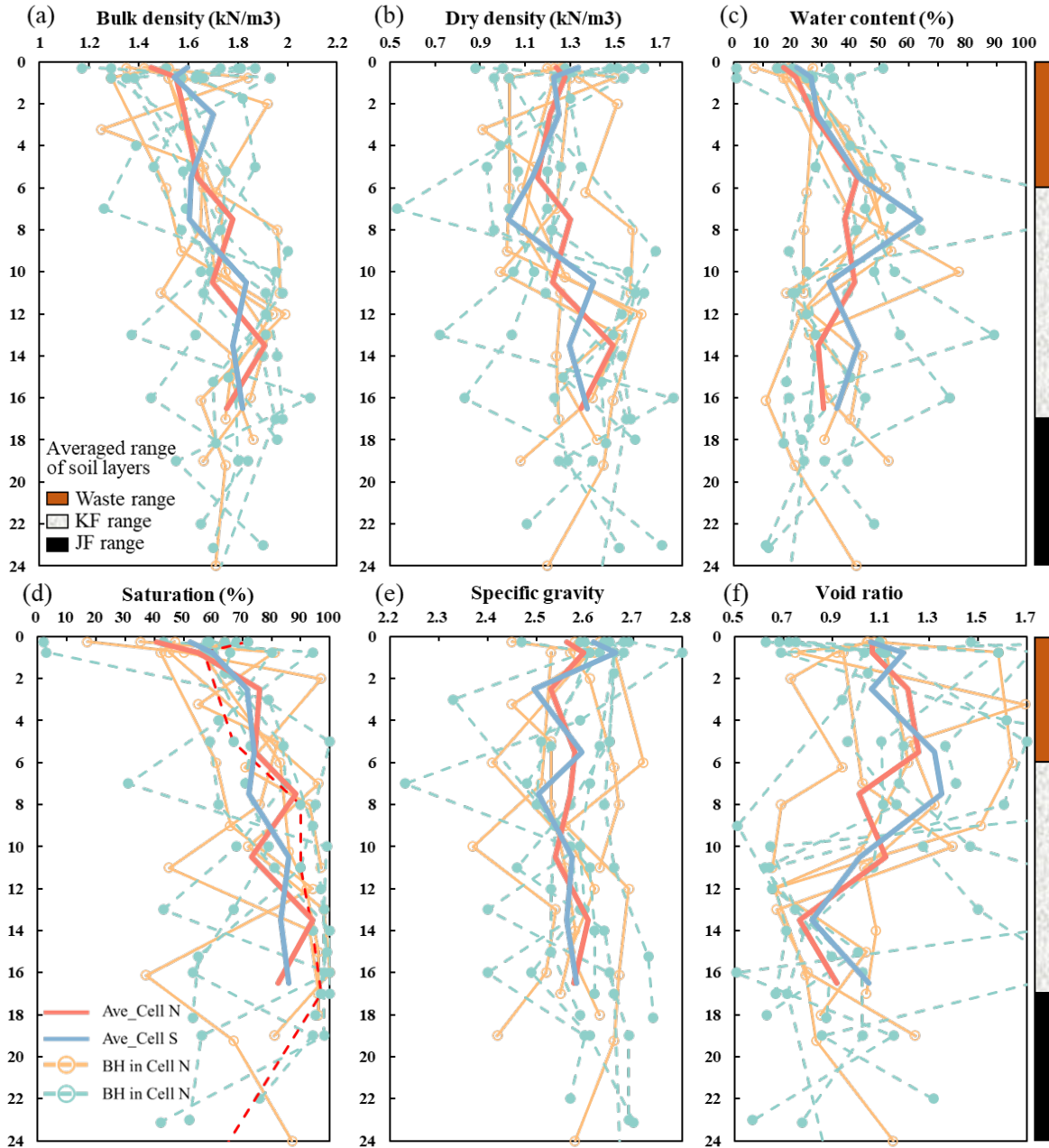
Fig. 6. Geotechnical properties of the waste retrieved from different depths: (a) bulk density; (b) dry density; (c) water content; (d) saturation degree; (e) specific gravity; (f) void ratio.
