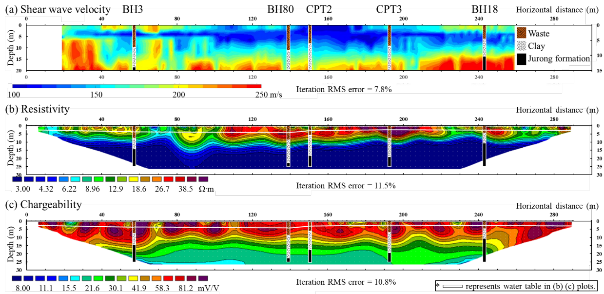
Fig. 7. 2D inversion results of the Cell S A1-G1 cross-section: (a) V_s plot based on MASW and MAM inversion results; (b) Res plot based on ERT inversion results; (c) IP plot based on IP inversion results.
