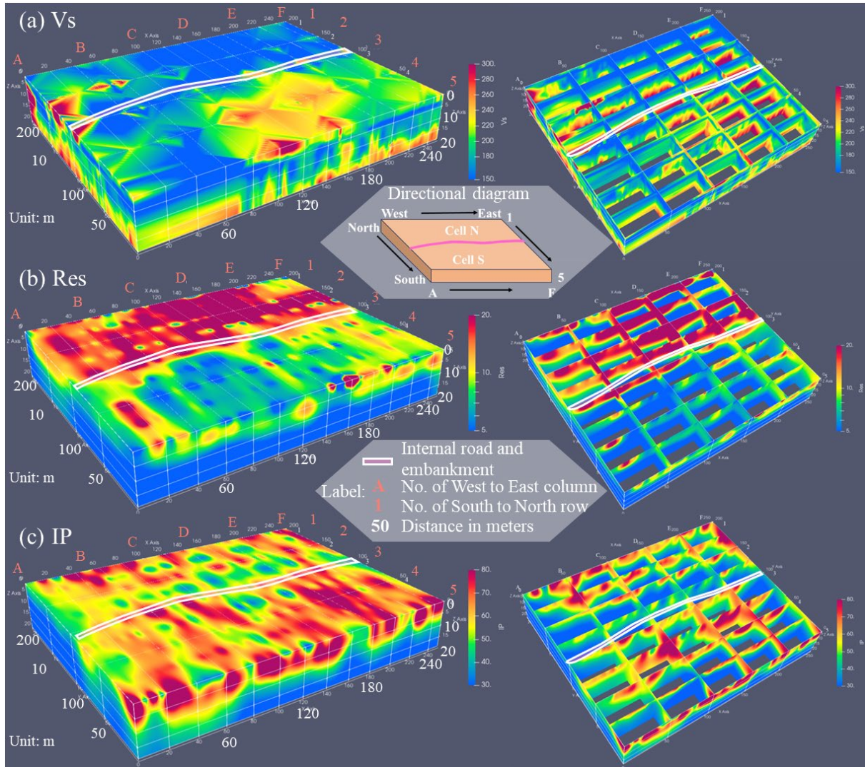
Fig. 8. 3D inversion results of Cell N and Cell S: (a) V_s profile; (b) Res profile; (c) IP profile.
