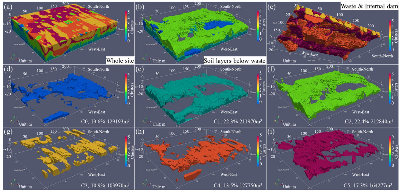
Fig 9. Waste stratification results using the K-means clustering method: (a) whole investigated zone; (b) soil layers below wastes; (c) waste layers and the internal dam; (d) C0 weathered rock layer in JF; (e) C1 bottom stiff clay layer in KF; (f) C2 shallow clay layer in KF; (g) high IP waste layer; (h) stiff waste layer; (i) high res waste layer.
