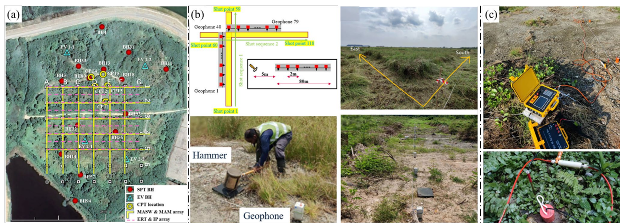
Fig. 2. Site information and geophysical investigation setup: (a) geophysical investigation plan and test locations; (b) MASW and MAM equipment; (c) ERT and IP equipment.
