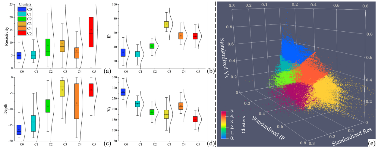
Fig 10. Statistical analyses of the K-means clustering results of Cell N and Cell S for (a) Res; (b) IP; (c) depth; (d) V_s ; and (e) distribution of all the geophysical measurements in 3D space.
