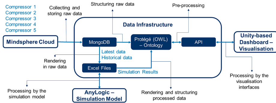
Fig. 14. DT data access and infrastructure.
