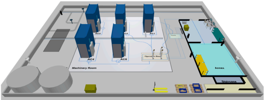
Fig. A2. AnyLogic 3D representation of the compressor station within the industrial facility's shop floor layout.
