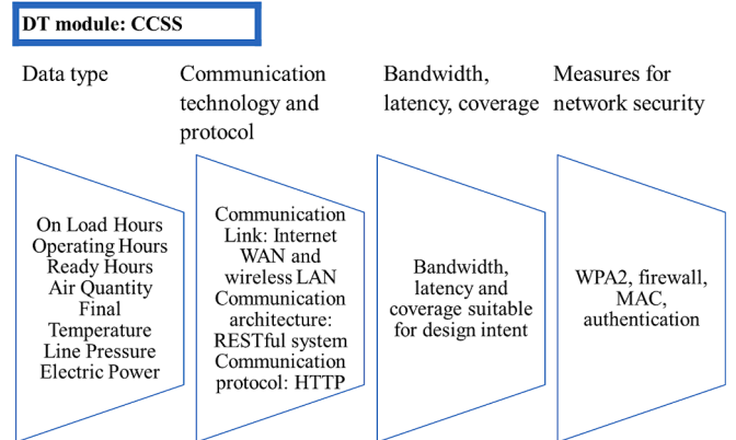
Fig. 10. DT communication network of the CCSS module.
