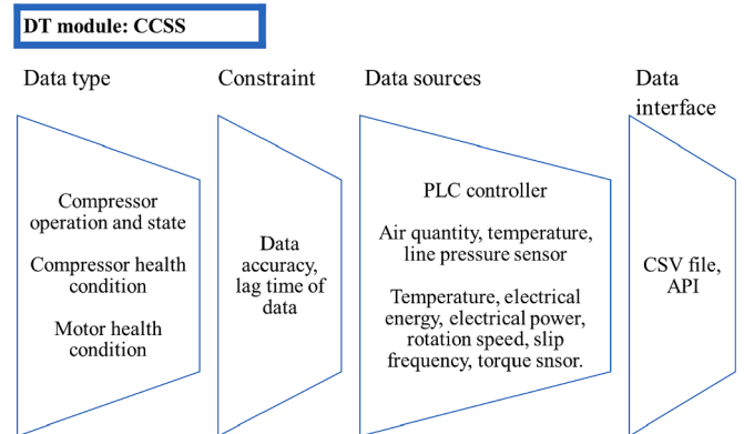
Fig. 6. DT data for the CCSS module.
