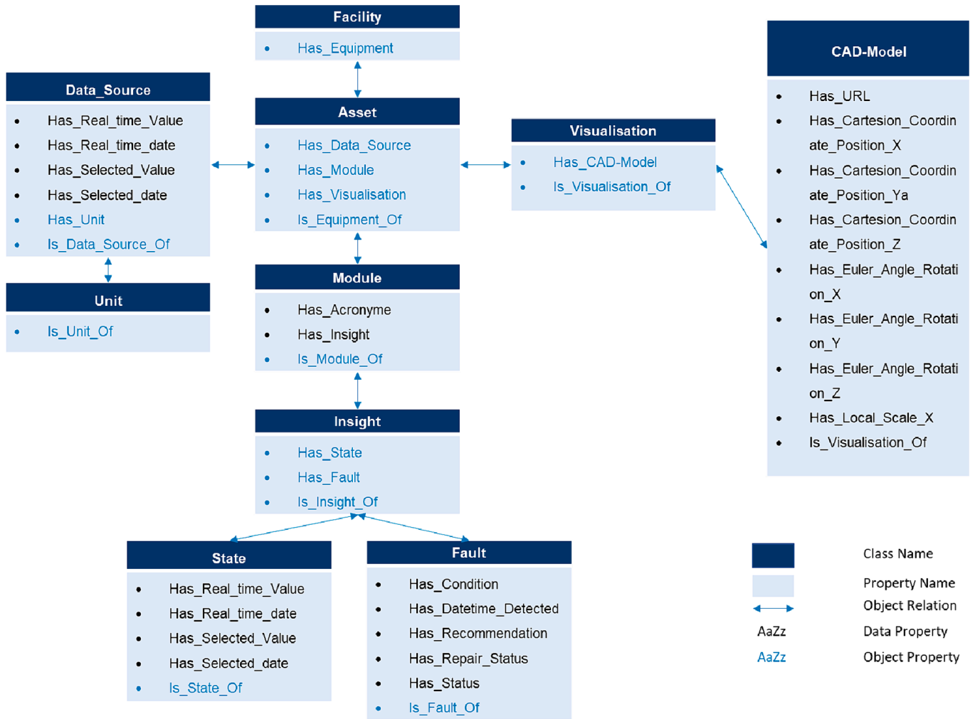
Fig. 12. UML class diagram of the ontology for the DT CCSS module.
