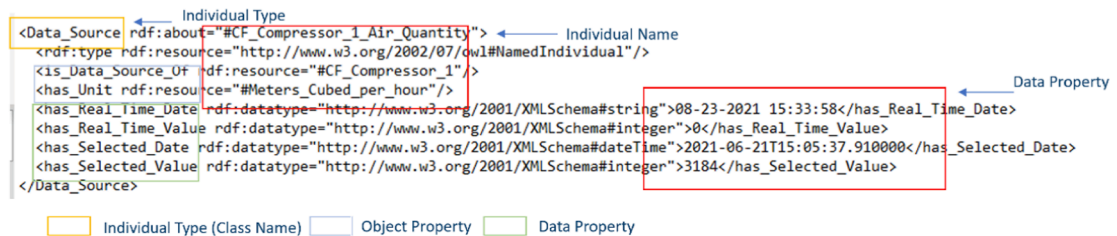
Fig. A1. Sample of data structure in OWL format.
