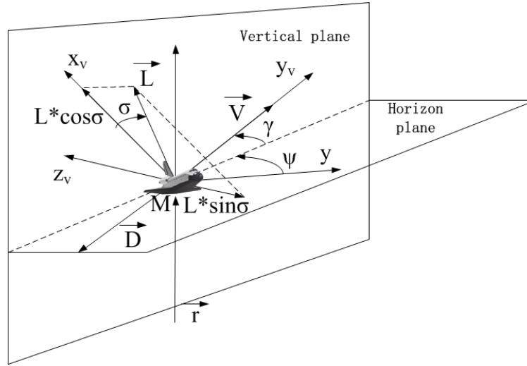
Figure 2. Aerodynamic forces
