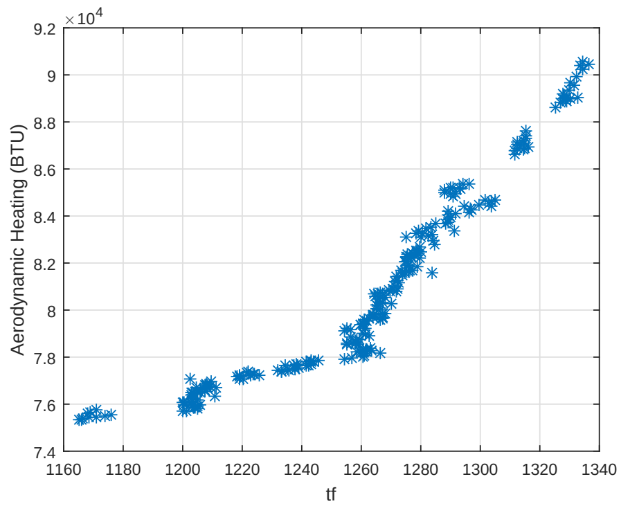
Figure 3. Pareto front obtained via extended NSGA-II
