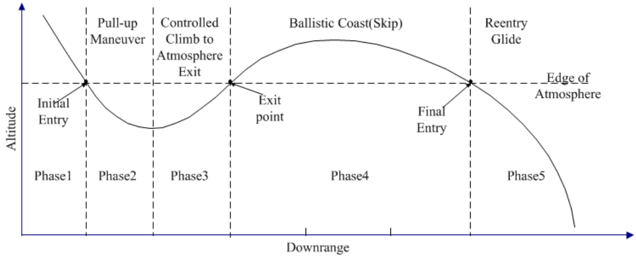
Figure 1. Mission profile
