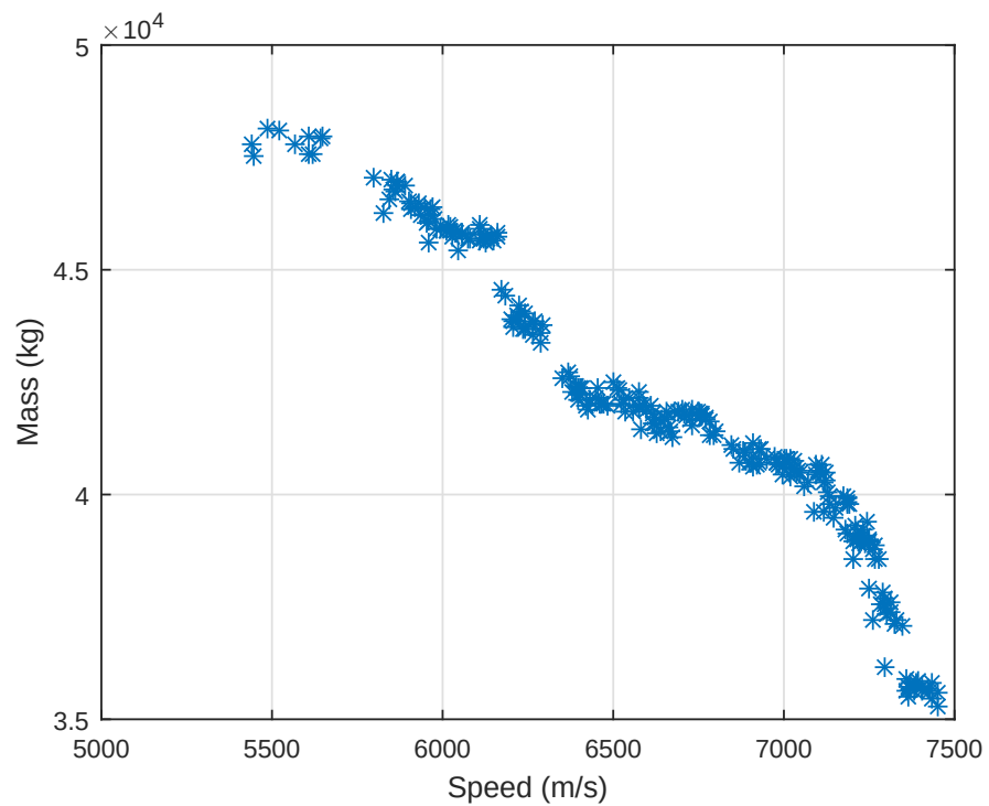
Figure 4. Pareto front obtained via extended NSGA-II
