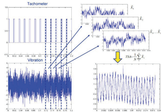
Figure 2 TSA layout [15]
