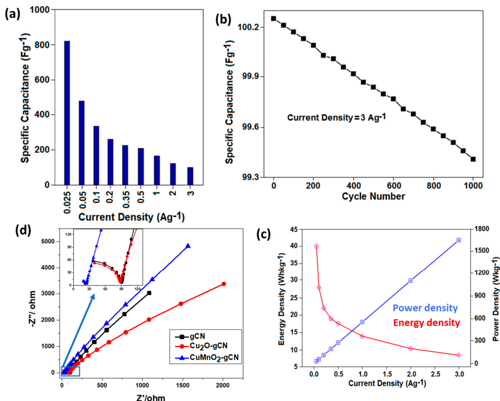
Figure 7. (a) Calculated specific capacitance of the \text{CuMnO}_2\text{-gCN} sample. (b) Cycling stability performance of \text{CuMnO}_2\text{-gCN} (the current density is 3 \text{ A}\cdot\text{g}^{-1} ). (c) The graphical relation between the energy density and power density as the function of current density for \text{CuMnO}_2\text{-gCN} material, in the potential range of 3.0–0.1 V. (d) Nyquist plots of gCN, \text{Cu}_2\text{O-gCN} , and \text{CuMnO}_2\text{-gCN} in a frequency range of 3 MHz–10 Hz under an open circuit condition.
