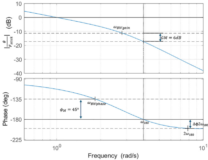
Figure 7. Definition of bandwidth and phase delay criteria [70].
