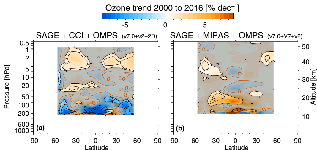
Figure 3. Same as Fig. 2, but showing the 2000 to 2016 ozone trends for the merged SAGE–ESA Ozone CCI–OMPS, and SAGE–MIPAS–OMPS data sets. The SAGE–ESA Ozone CCI–OMPS data set uses the OMPS 2-D retrieval from U. Saskatoon. The SAGE–MIPAS–OMPS data set uses the OMPS v2 retrieval from NASA.
