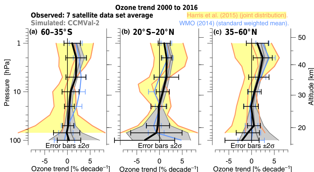
Figure 5. Same as Fig. 4, but giving the average 2000 to 2016 ozone trends (black lines) from seven merged satellite data sets (GOZCARDS, SWOOSH, SAGE–OSIRIS, SAGE–CCI–OMPS(2D), SAGE–MIPAS–OMPS(v2), SBUV–NASA, and SBUV–NOAA). SBUV trends are only used at levels above 40 hPa (23 km). For comparison, the 1998 to 2012 average ozone trend from Harris et al. (2015, yellow lines and shading), and the 2000 to 2013 average ozone trend from WMO 2014 (blue lines) are shown as well. In all cases, uncertainty bars or shading give \pm 2\sigma uncertainty. For the 2000 to 2016 satellite average ozone trends (black error bars), and trends from Harris et al. (2015, yellow shading) the uncertainty is derived from the SD \sigma between individual trends in the average (joint distribution case). For the WMO 2014 trends (blue error bars), the uncertainty of the standard weighted mean is given (see text for details). Grey lines and shading give the trend and \pm 2\sigma uncertainty obtained from multimodel mean and SD of the CCMVal-2 model simulations (see text in Sect. 4.1).
