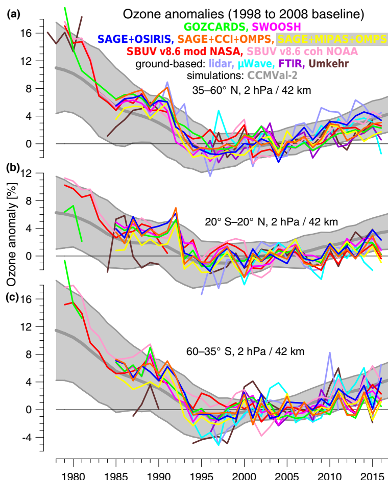
Figure 1. Annual mean ozone anomalies near 2 hPa or 42 km, as recorded by merged satellite data sets and ground-based stations. Anomalies are referenced to the 1998 to 2008 climatological annual cycle of each individual data set, and are averaged over the indicated zonal bands. Stations close to a zonal band are also included, i.e., NDACC lidar data from Table Mountain at 34.4° N, NDACC FTIR data from Izaña at 28.3° N and Wollongong at 34.4° S, and Umkehr data from Perth at 34.7° S are included in the respective midlatitude bands. Due to contamination by volcanic aerosol after the eruptions of El Chichon and Mt. Pinatubo, Umkehr data are not used for the years 1982, 1983, and 1991 to 1993, and SBUV-NASA data are not available for 1992. Grey lines show the multimodel mean ozone anomalies from CCMVal-2 simulations (Eyring et al., 2010), with the grey shading giving the \pm 2 SD envelope. Mean and SD are taken over all models (except outliers) and within a 25-month sliding window.
