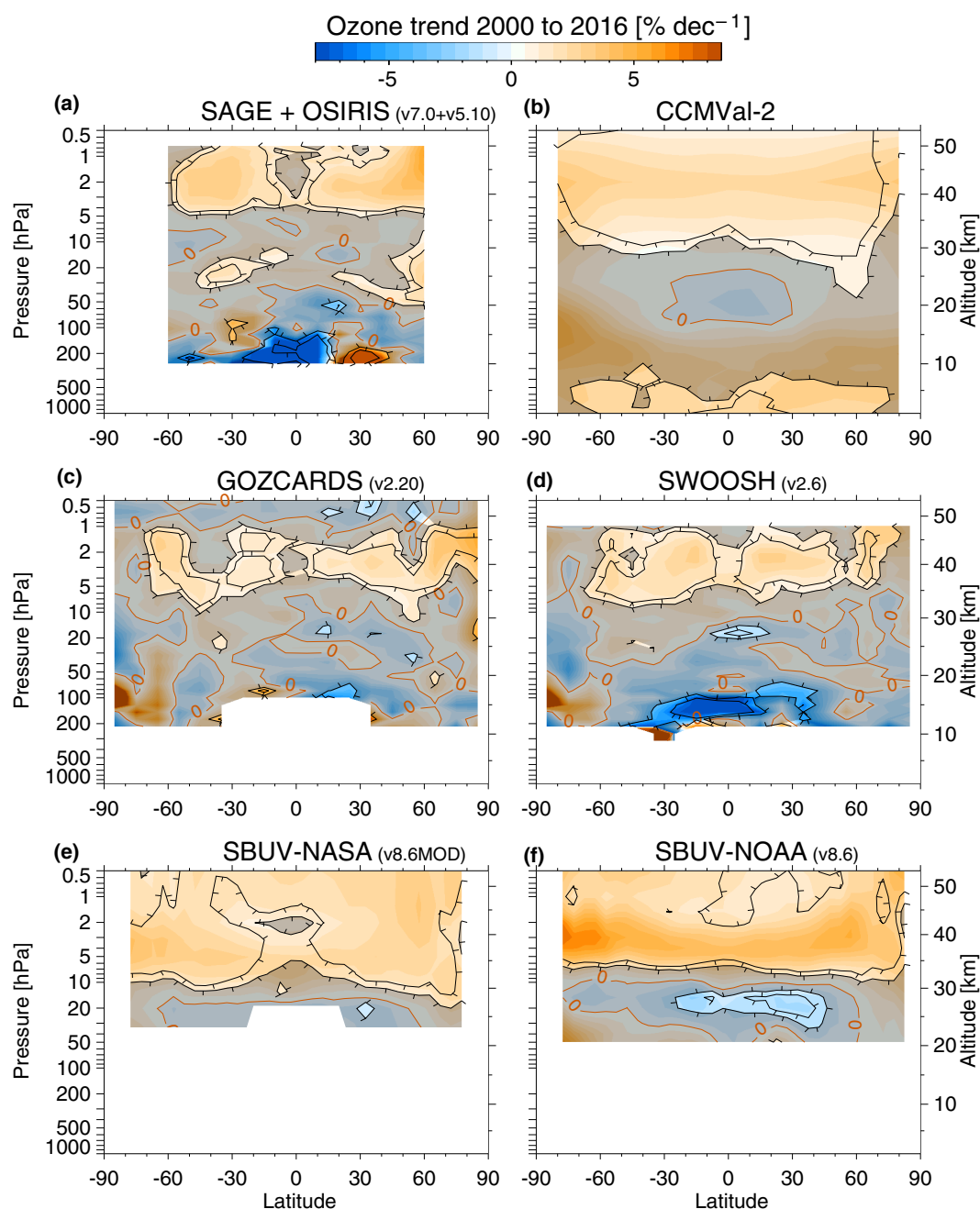
Figure 2. Latitude pressure cross section of 2000 to 2016 ozone trends TR obtained by 2-step multiple linear regression (see text). Panel (b) is for model simulations from the CCMVal-2 initiative. The other panels are for merged satellite data sets. The colour scale gives trend magnitude TR. Shading and isolines give the ratio of trend to trend uncertainty, |TR|/\sigma . Grey shading, in regions where |TR| \leq 2\sigma , indicates that trends are not significant at the 95 % confidence level. The next isoline is at |TR|/\sigma = 3 .
