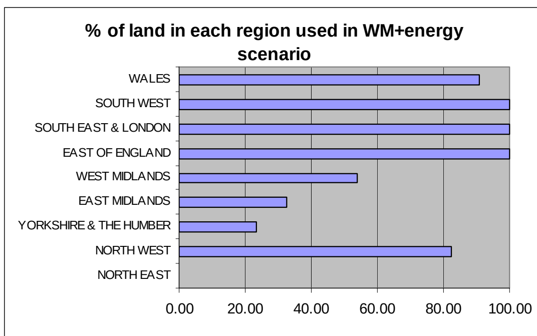
Figure 4.4 : Regional distribution of lowland land used for intensive farming for WM Scenario, 2050
