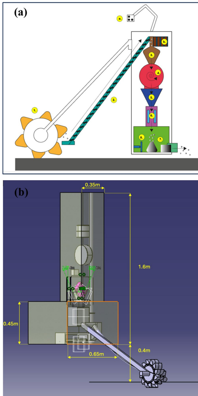
Fig. 3 a Simple schematic presentation of the material handling experimental payload with subsystems presented with different colours: (1.) bucket wheel, (2.) screw conveyer, (3.) sieve, (4.) rotating drum, (5.) wedge hopper, (6.) electrostatic plates, (7./8.) container with linear actuator, (a.) robotic arm, (b.) carousel dosing device for Earth samples. b is an indicative computer aided design (CAD) representation of packaging the developed version of the payload within payload accommodation volumes of Blue Ghost lander
