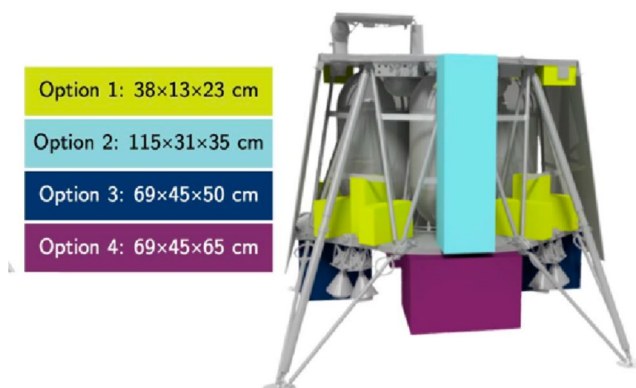
Fig. 4 Blue Ghost lander with available payload bay options highlighted (credit: Firefly Aerospace)
