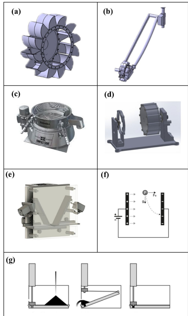
Fig. 2 Schematic presentation of subsystems to be installed in baseline payload: a Excavation—Bucket Wheel, b Conveying—screw conveyor, c sorting—sieve (credit: Russell Finex Ltd.), d dynamic handling—rotating drum, e static handling—wedge hopper, f electrostatic separation, g container for pile forming, and linear actuator for compressing
