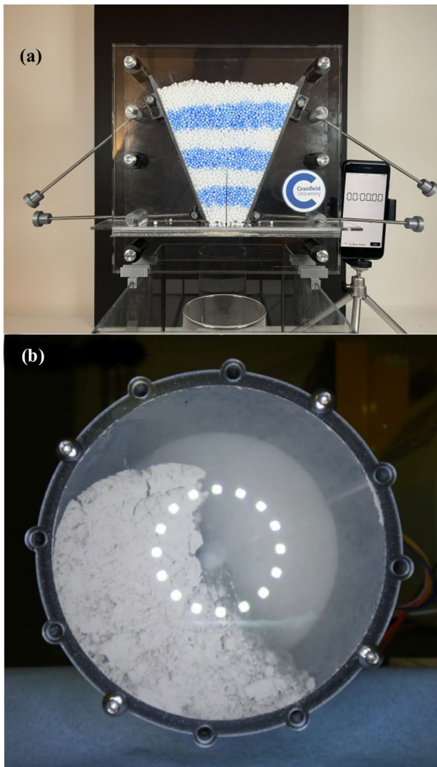
Fig. 1 a A simple laboratory breadboard version of wedge hopper with a manual adjustable inclined walls and discharge outlet. This example is filled with white and blue expanded polystyrene beads. The beads are 2 mm in diameter and hopper is 250 \times 250 \times 40 mm in dimension. Video frame b Rotating drum with 80 mm external diameter and 30 mm of depth, with adjustable rotating speeds, for test filled with NU-LHT-2 M lunar regolith simulant (Zanotti et al. 2024). Transparent vertical walls allow video recording of the granular material behaviour
