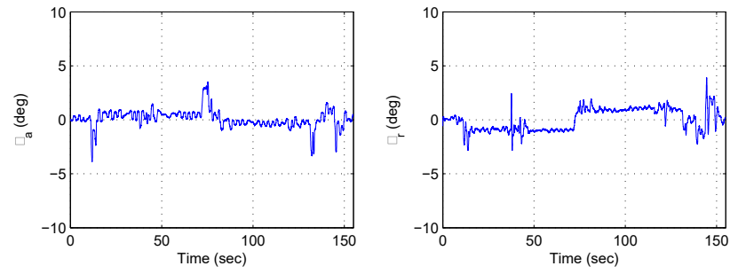
(b) Control surface deflections
