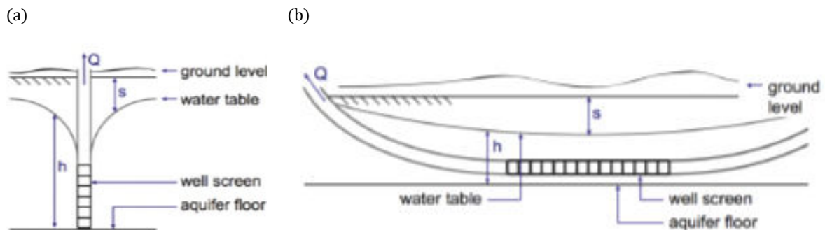
Figure 1. Comparison of scheme of (a) vertical and (b) horizontal remediation well operating with a pumping rate, Q , in an unconfined aquifer. Both wells configurations incur a surrounding hydraulic head, h , field with drawdown profile, S .
