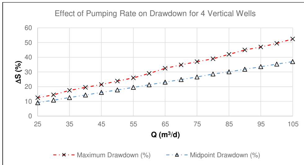
Figure 8. Multiple VRW configuration results of percentage drawdown by varying the pumping rate and the hydraulic head between four 12" diameter vertical wells, placed at x = 2.5 \text{ m} , y = \pm 2 \text{ m} , \pm 6 \text{ m} .
