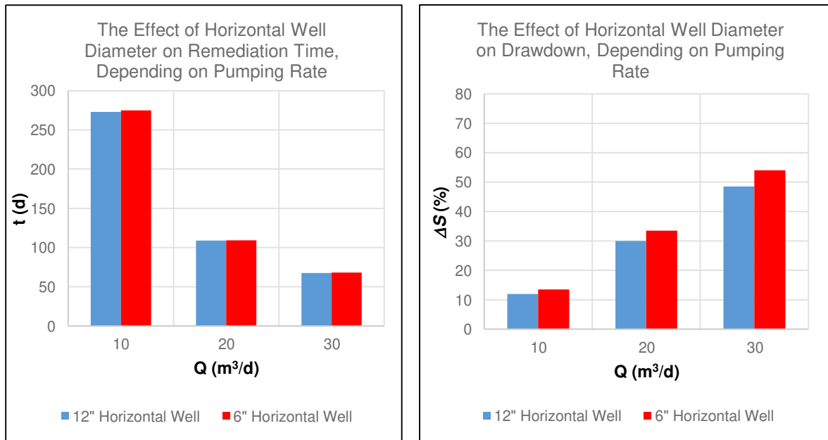
Figure 4. Comparison of remediation times between two well diameters respectively for (a) vertical and (b) horizontal wells.
