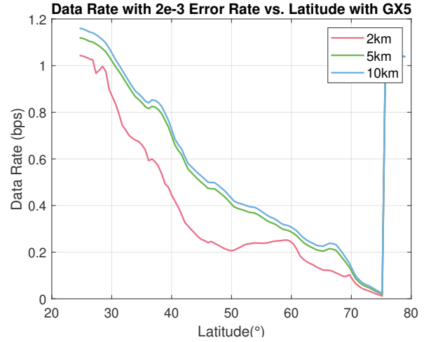
Fig. 7. Data rate in function of latitude and aircraft altitude
