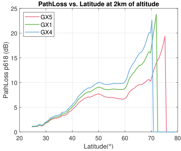
Fig. 5. Path Losses against the Latitude of Aircraft
