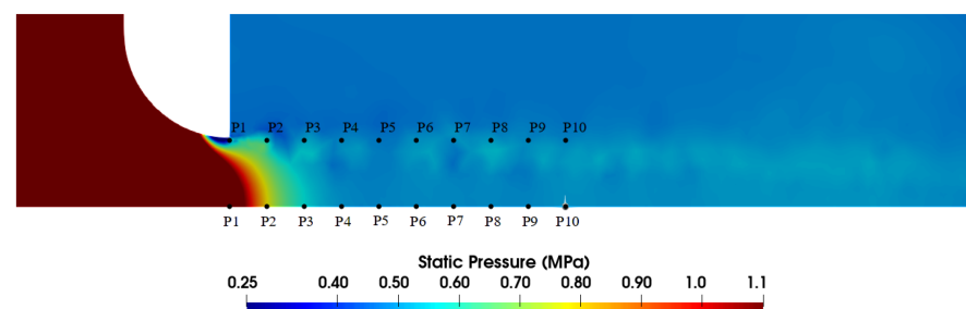
Figure 9. Static pressure field around the orifice, with pressure data probes displayed showing the region of low pressure around the orifice.
