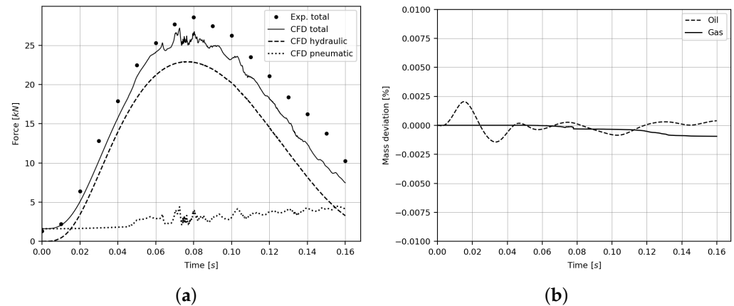
Figure 4. Shock absorber case validation: (a) force validation; (b) mass conservation of the oil and gas phases.
