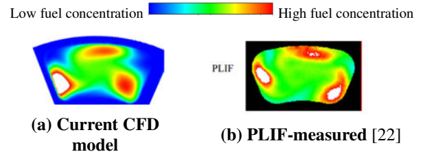
Figure 6. Fuel distribution at the main nozzle exit of the present study and Ref [22]
