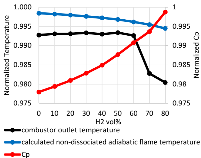
Figure 15 Normalized temperature (combustor outlet and calculated non-dissociated adiabatic flame temperature) and specific heat for different H_2/CH_4 blends
