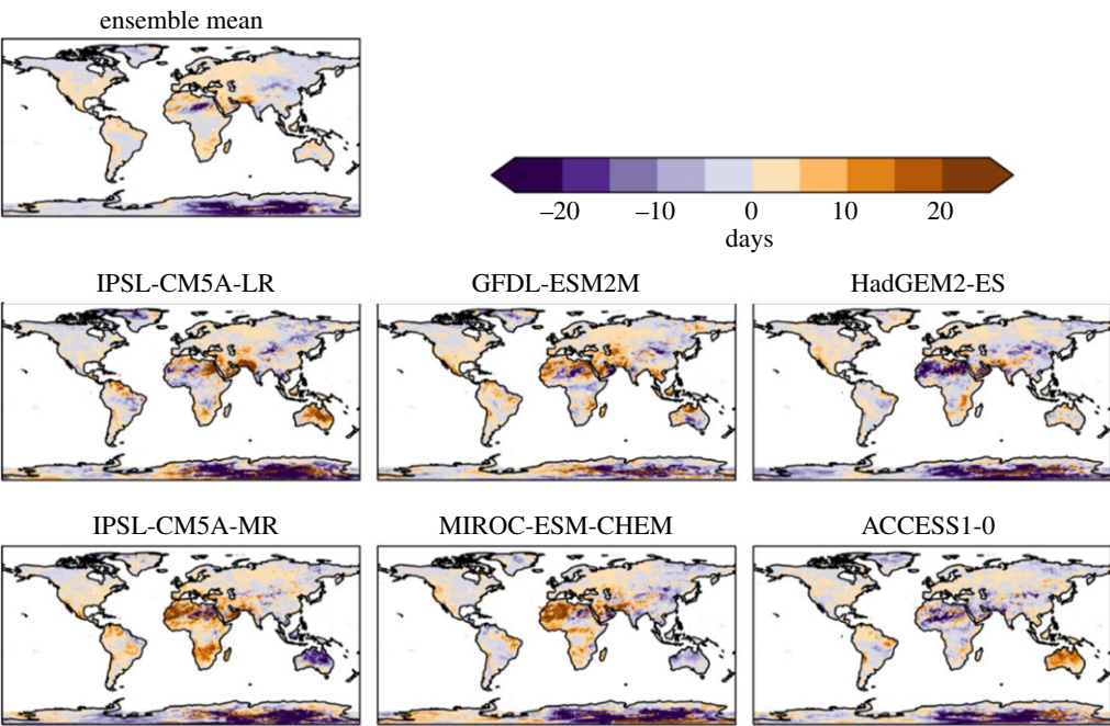
Figure 16. Difference in consecutive dry days between 2°C and 1.5°C global warming, for individual ensemble members and ensemble mean.
