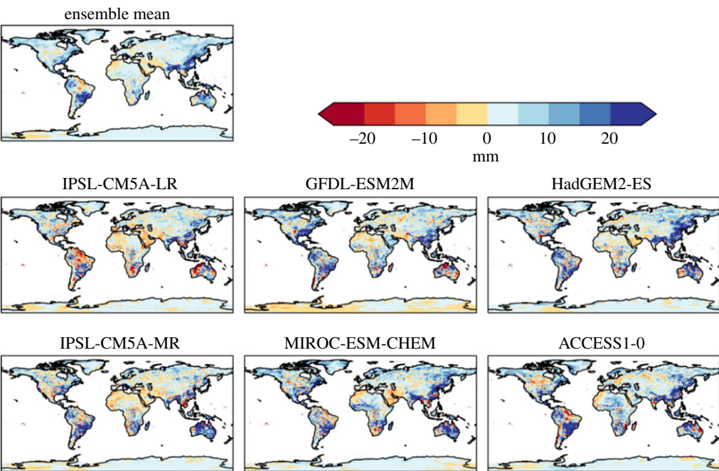
Figure 17. Difference in annual maximum 5 day rainfall between 2°C and 1.5°C global warming, for individual ensemble members and ensemble mean.
