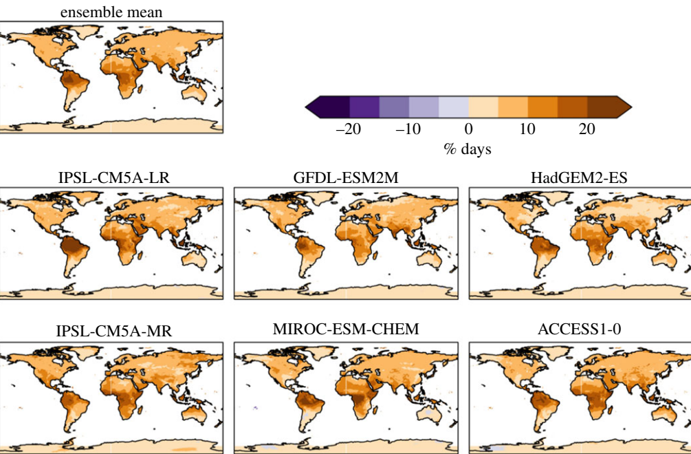
Figure 15. Difference between 2°C and 1.5°C global warming for percentage of days with maximum temperature above 90th percentile of baseline, for individual ensemble members and ensemble mean.
