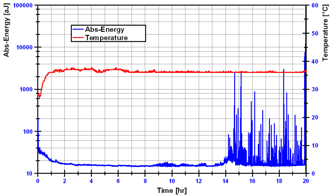
Figure 11 Test conditions run until visually observable surface damage
