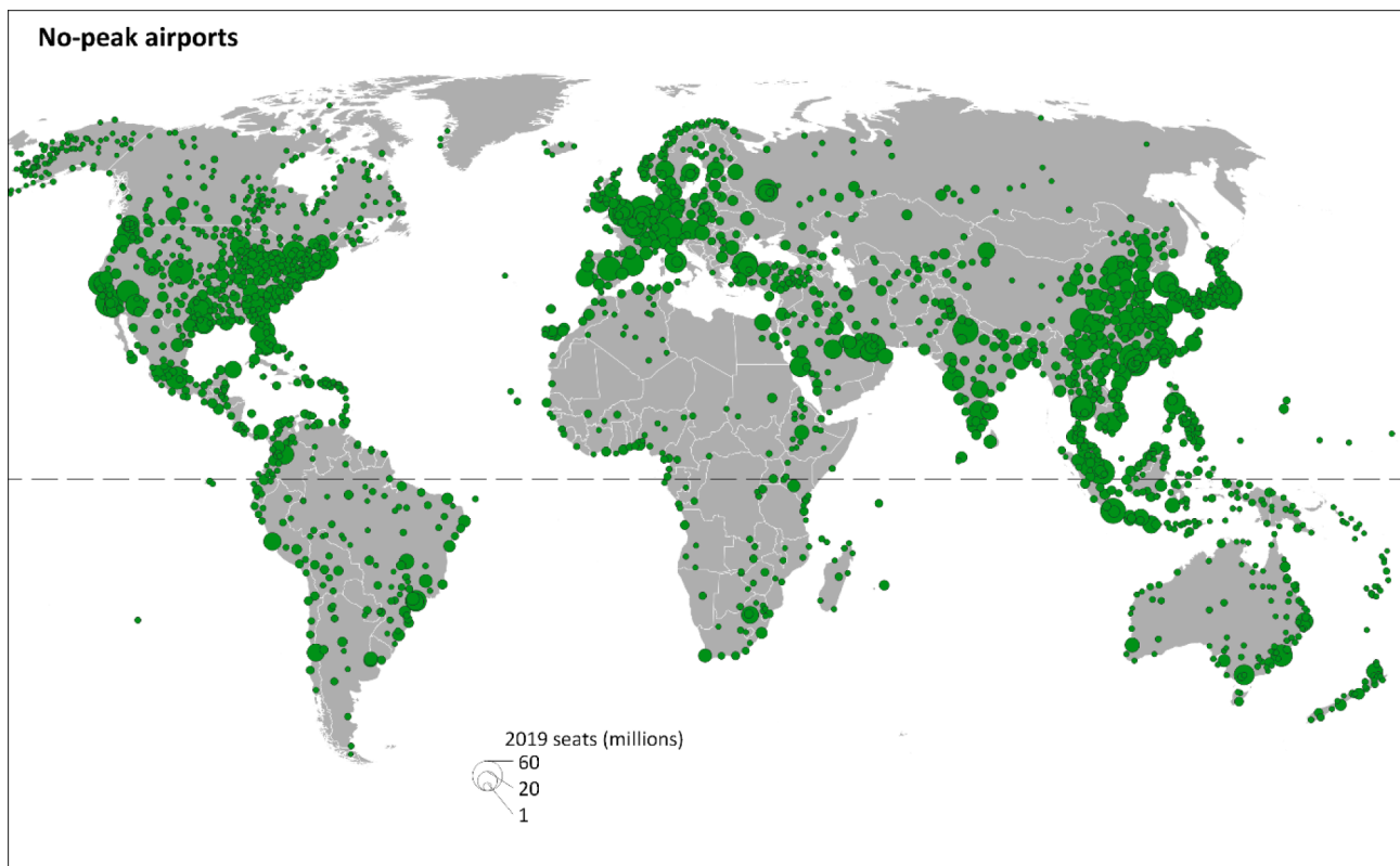
Fig. 6. No-peak airports.
