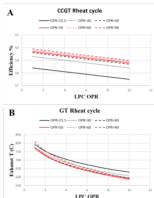
Figure 8. (A) Effects of the compression ratio with changing LPCs in the reheat CCGT cycle. (B) Effects of the compression ratio with changing LPCs in the reheat GT cycle.
