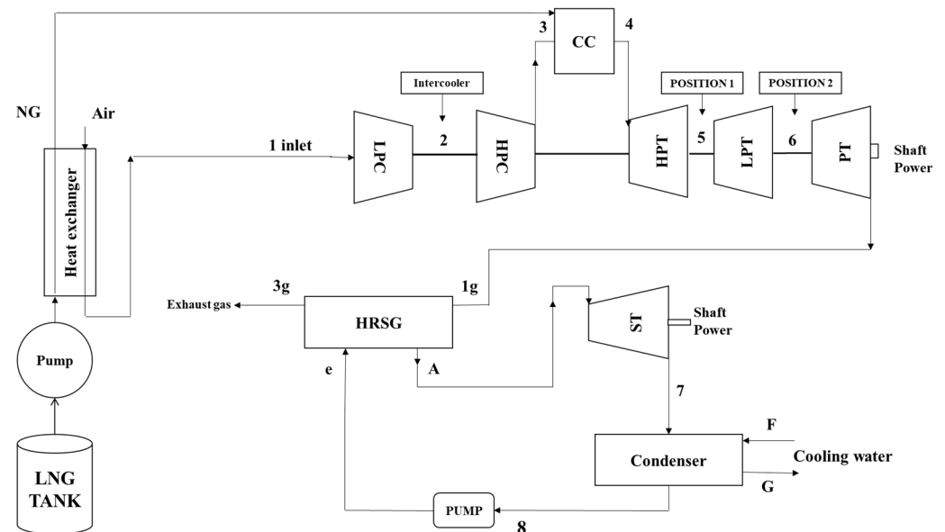
Figure 4. ELNG cycle layout. LNG: liquefied natural gas; HPC: high-pressure compressor; LPC: low-pressure compressor; CC: combustion chamber; S.T.: steam turbine; 1: outlet air mass flow temperature from heat exchanger to low-pressure compressor; NG: the outlet natural gas mass flow from heat exchanger to combustion chamber.
