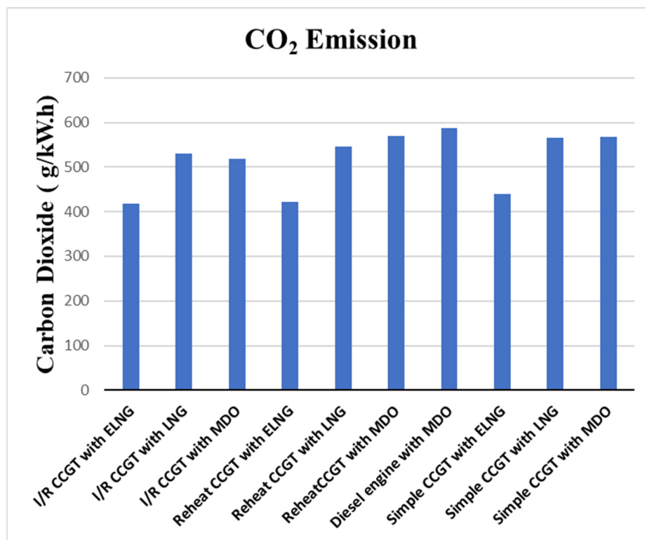
Figure 15. CO 2 emissions from all propulsion systems.
