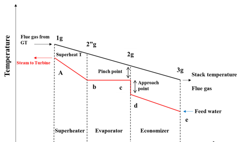
Figure 3. Temperature diagram of the heat recovery steam generator (HRSG); A: outlet steam mass flow temperature from HRSG to steam turbine; b and c: temperature of the steam inlet and outlet the evaporator; d: outlet fluid mass flow temperature from economizer.
