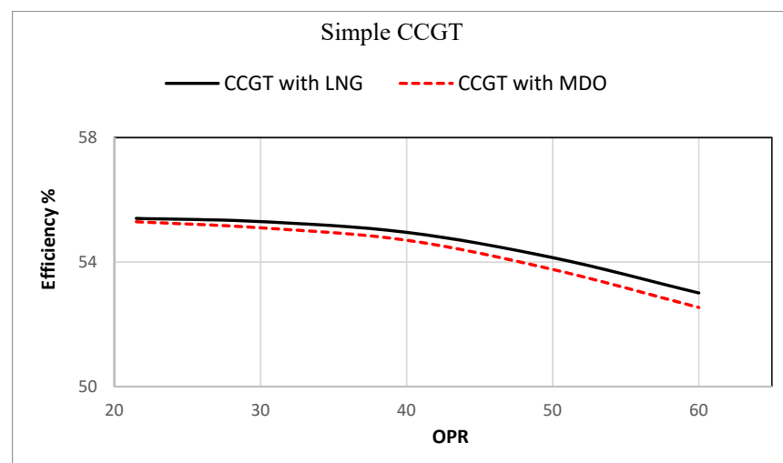
Figure 6. Effects of the compression ratio on the overall thermal efficiency. MDO: marine diesel oil; OPR: overall pressure ratio.
