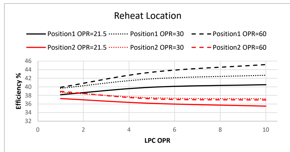
Figure 7. Effects of the compression ratio with different LPCs in the reheat cycle.
