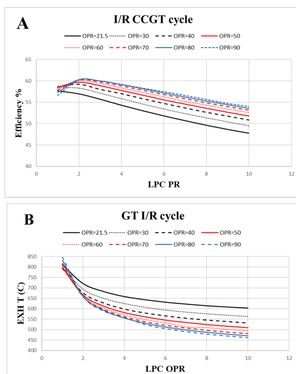
Figure 9. (A) Effects of the compression ratio with changing LPC in the I/R CCGT cycle. (B) Effects of the compression ratio with changing LPC in the I/R GT cycle.
