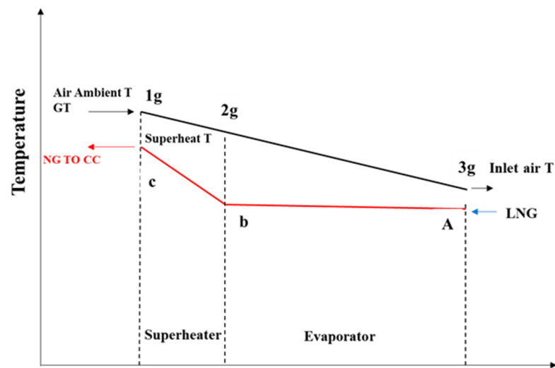
Figure 5. Heat balance in the heat exchanger between LNG and inlet air. 1g: inlet air mass flow temperature to heat exchanger; 2g: outlet air mass flow temperature from superheater stagnation to evaporator; 3g: outlet air mass flow temperature from heat exchanger to gas turbine; A: inlet LNG mass flow temperature to heat exchanger; b: outlet LNG mass flow temperature evaporator stagnation to superheater; c: outlet NG mass flow temperature from heat exchanger to combustion chamber gas turbine.
