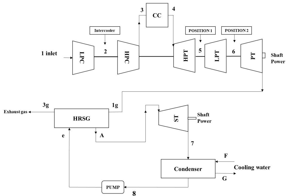
Figure 2. Flowchart of the CCGT model. HPT: high-pressure turbine; LPT: low-pressure turbine; P.T.: power turbine; HRSG: heat recovery steam generator; 1: inlet air mass flow temperature to low-pressure compressor; 2: outlet air mass flow temperature from low-pressure compressor to high-pressure compressor; 3: outlet air mass flow temperature from high-pressure compressor and inlet air mass flow to combustor; 4: outlet air-fuel mass flow temperature from combustor to high-pressure turbine; 5: outlet air-fuel mass flow temperature from high-pressure turbine to low-pressure turbine; 6: outlet air-fuel mass flow temperature from low-pressure turbine to power turbine; 1g: exhaust air-fuel mass flow temperature from gas turbine to HRSG; 3g: exhaust air-fuel mass flow temperature from HRSG; A: outlet steam mass flow temperature from HRSG to steam turbine; 7: outlet steam mass flow temperature from steam turbine to condenser; 8: outlet water mass flow temperature from condenser to the pump; e: outlet water mass flow temperature from pump to HRSG.
