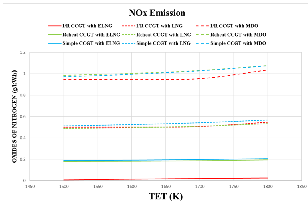
Figure 12. Effects of the TET on the NO x .
