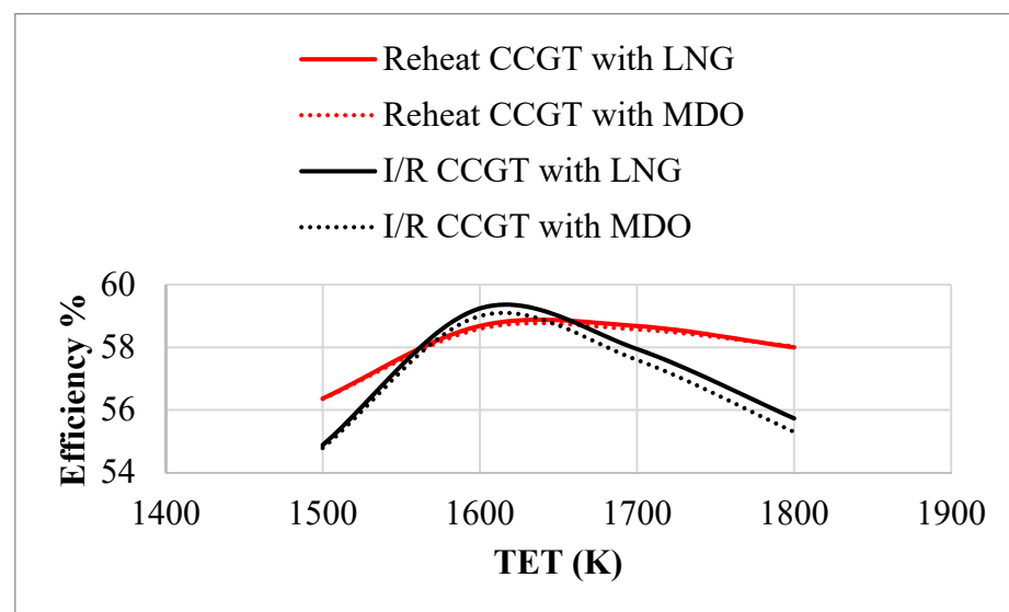
Figure 10. Effect of the TET on the overall thermal efficiency.
