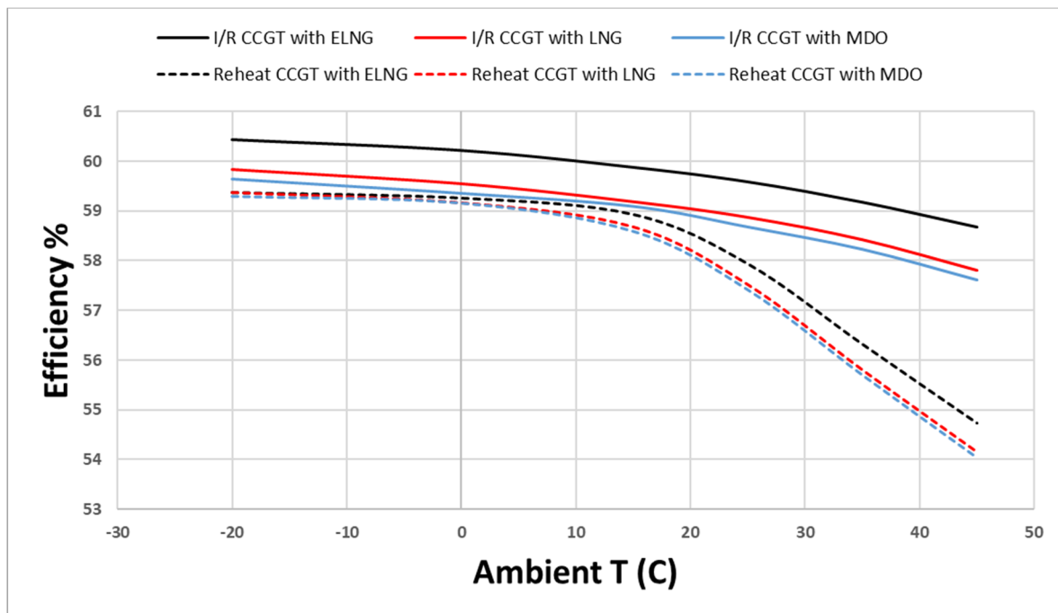
Figure 11. Effects of the ambient temperature on the overall thermal efficiency.
