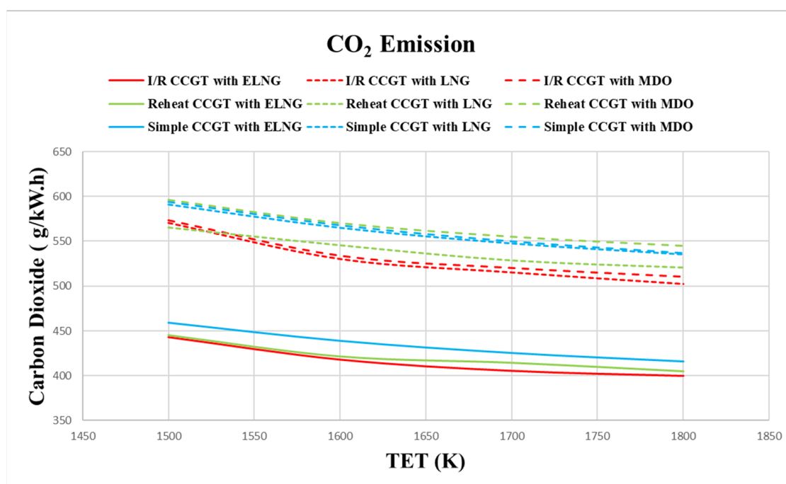
Figure 13. Effects of the TET on the CO 2 emissions.
