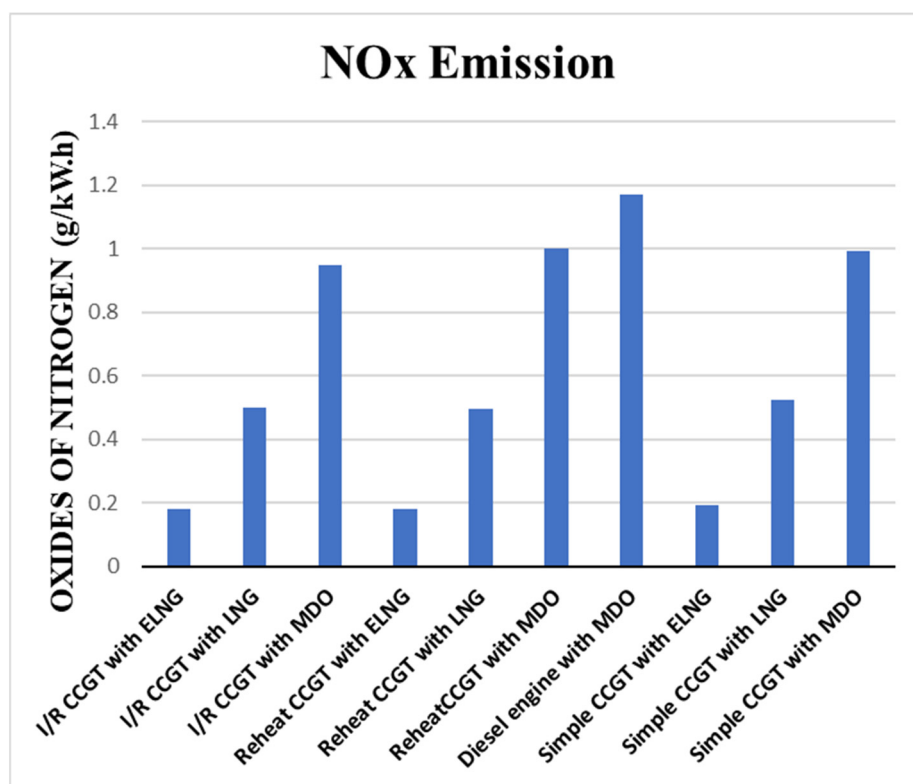
Figure 14. NO x emissions from all propulsion systems.
