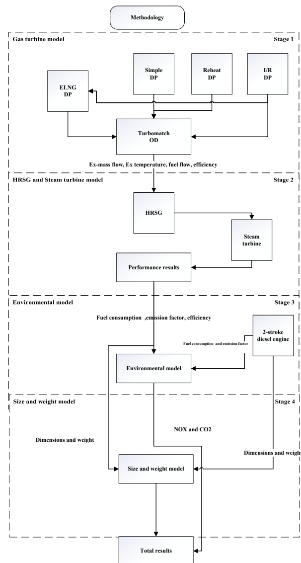
Figure 1. Flowchart of the methodology employed in this study. NO x : Nitrogen oxide; CO 2 : carbon dioxide; CCGT: combined-cycle gas turbine (with steam); I/R: intercooler–reheat cycle; HRSG: heat recovery steam generator; ELNG: enhanced liquefied natural gas.
