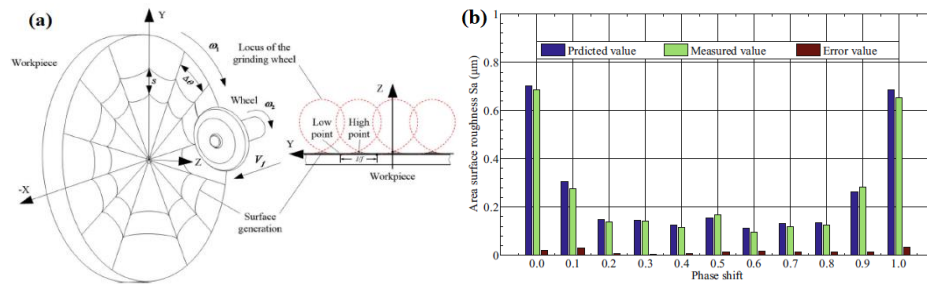
Fig. 20. Method and result in Chen's work. (a) Spiral marks generated by the wheel with micro-vibration and (b) comparison diagram between predicted and measured area surface roughness [95].
