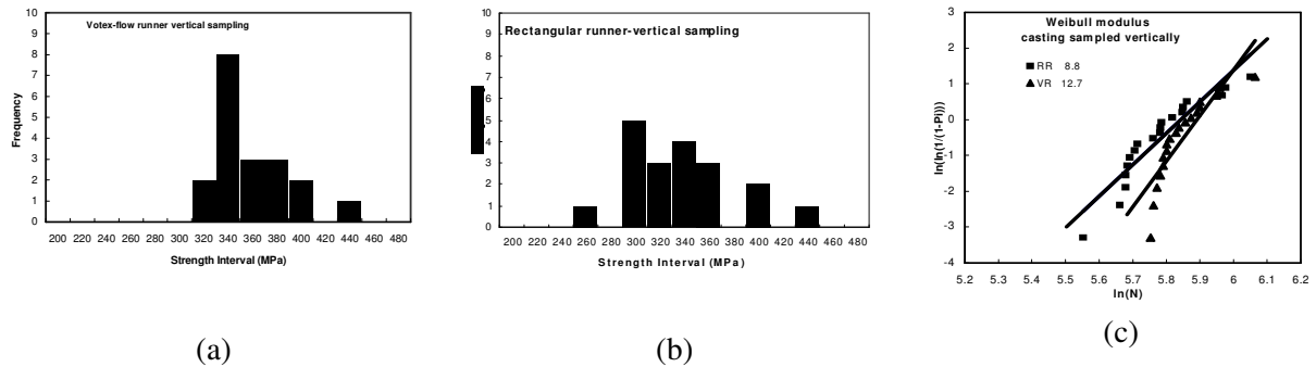
Figure 8. (a) UBS distributions of VR runner system; (b) UBS distributions of RR runner system; (c) Weibull plots of all the casting specimens UBS.
